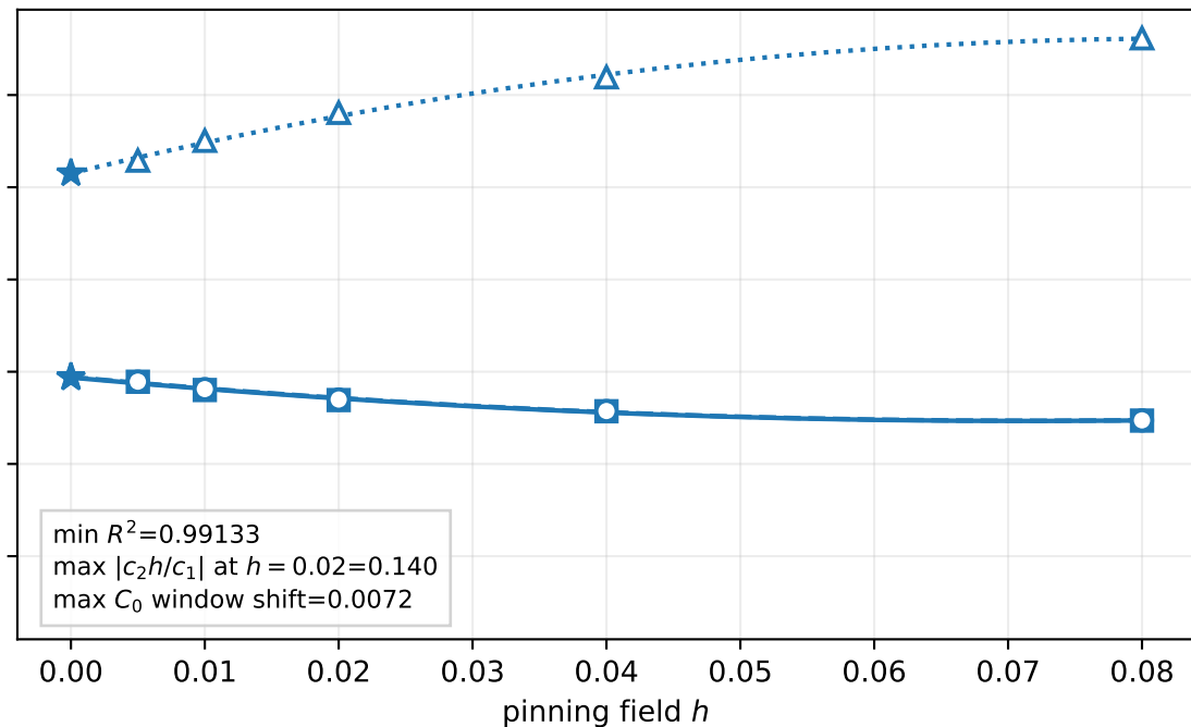
Plaquette pin
