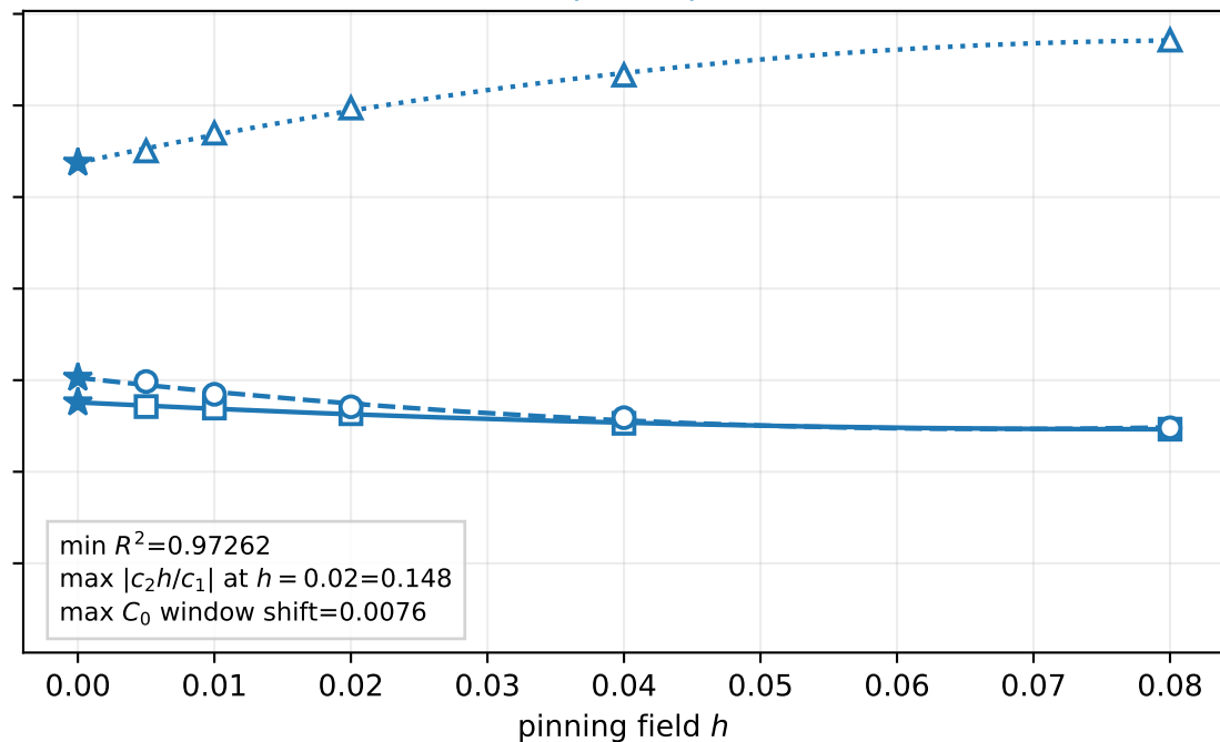
Plaquette pin
