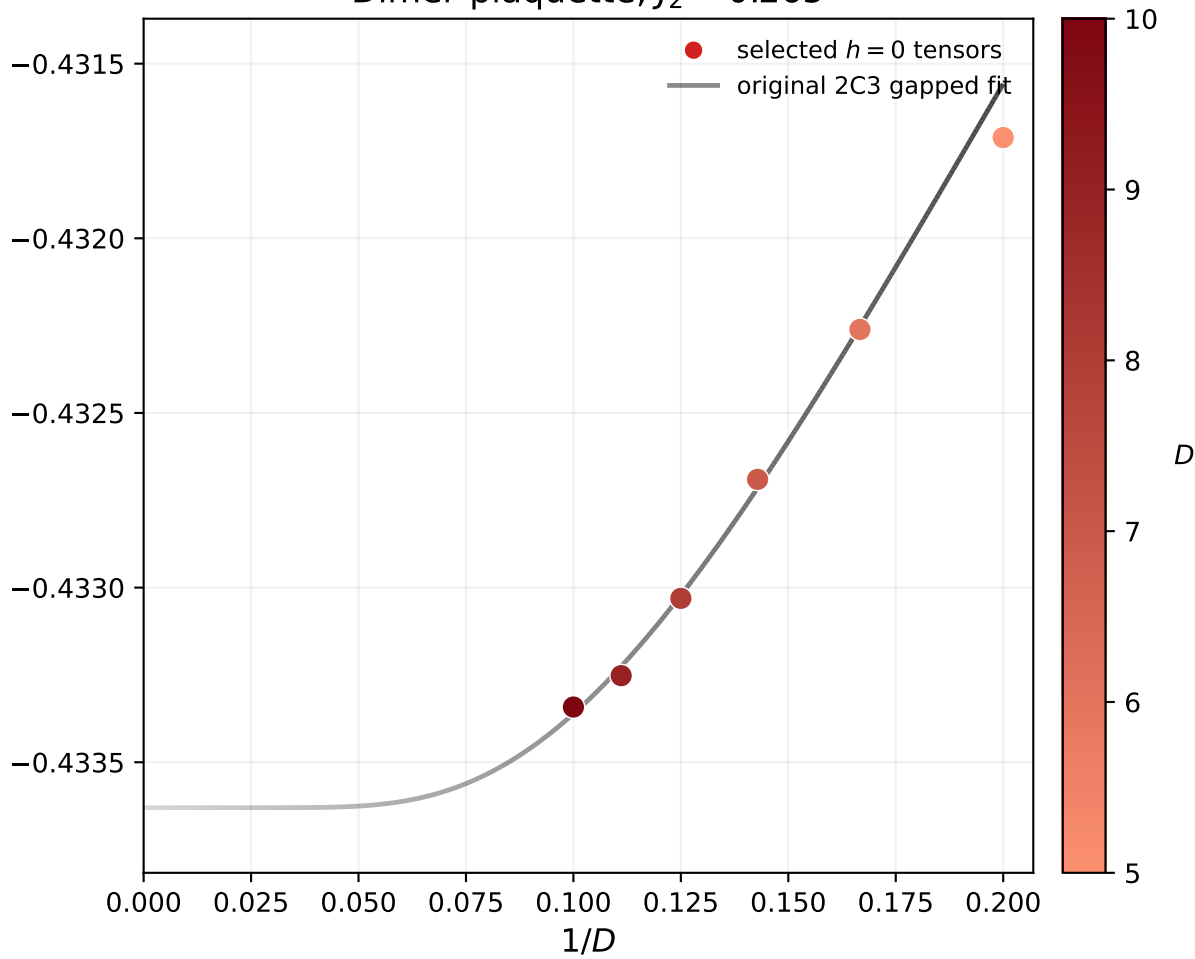
Dimer-plaquette, J_2 = 0.265
