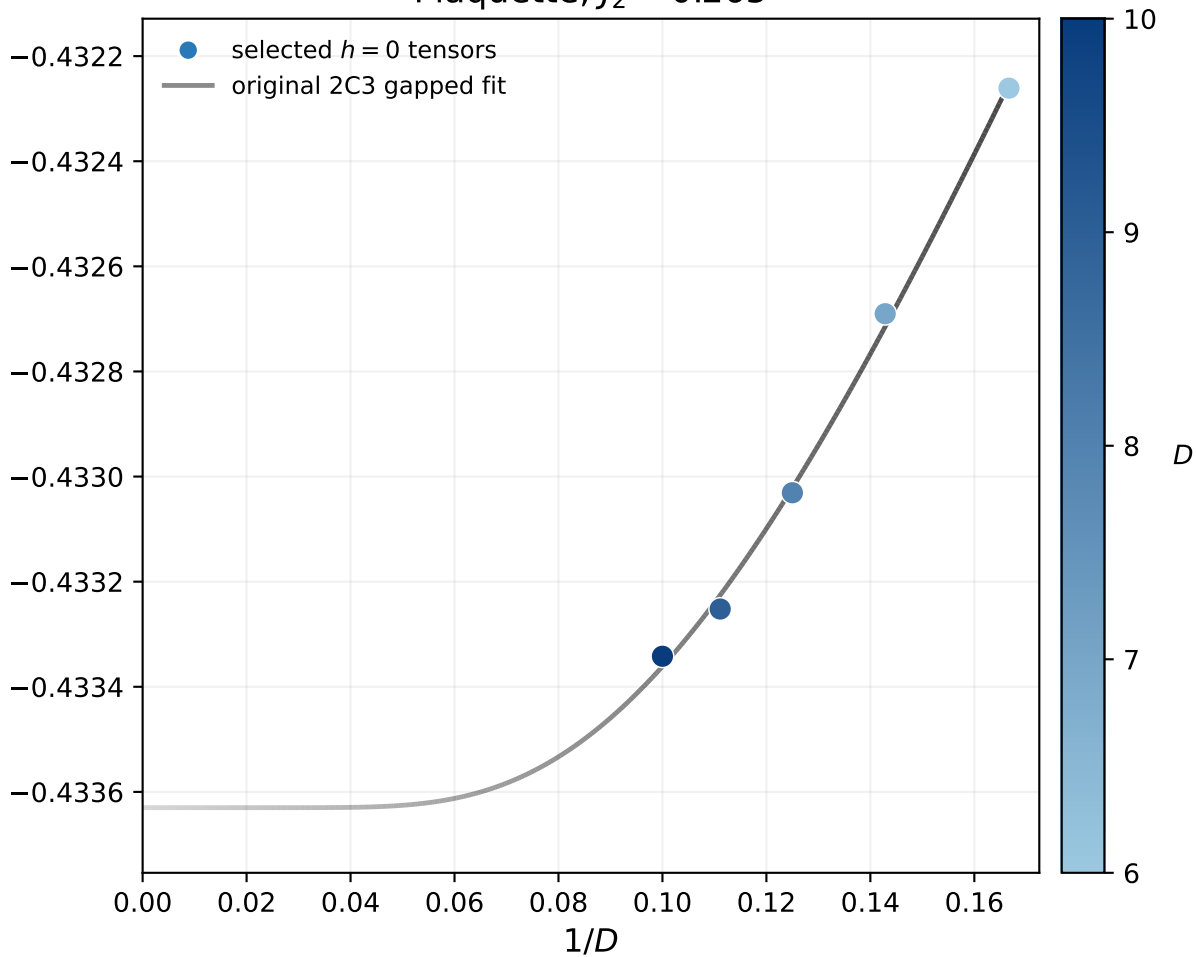
Plaquette, J_2 = 0.265
