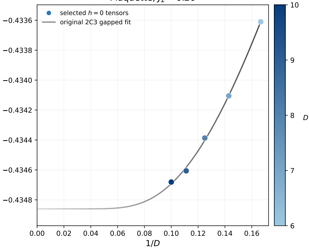
Plaquette, J_2 = 0.26
