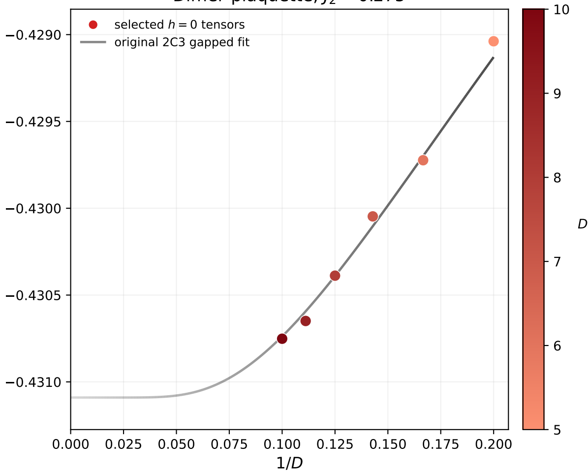
Dimer-plaquette, J_2 = 0.275
