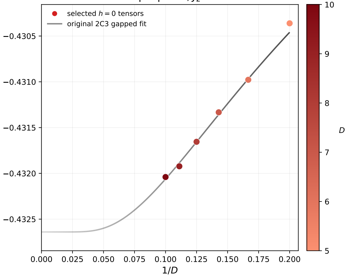
Dimer-plaquette, J_2 = 0.27
