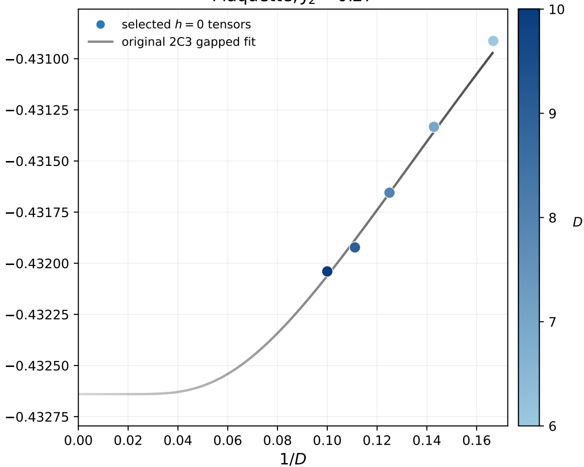
Plaquette, J_2 = 0.27
