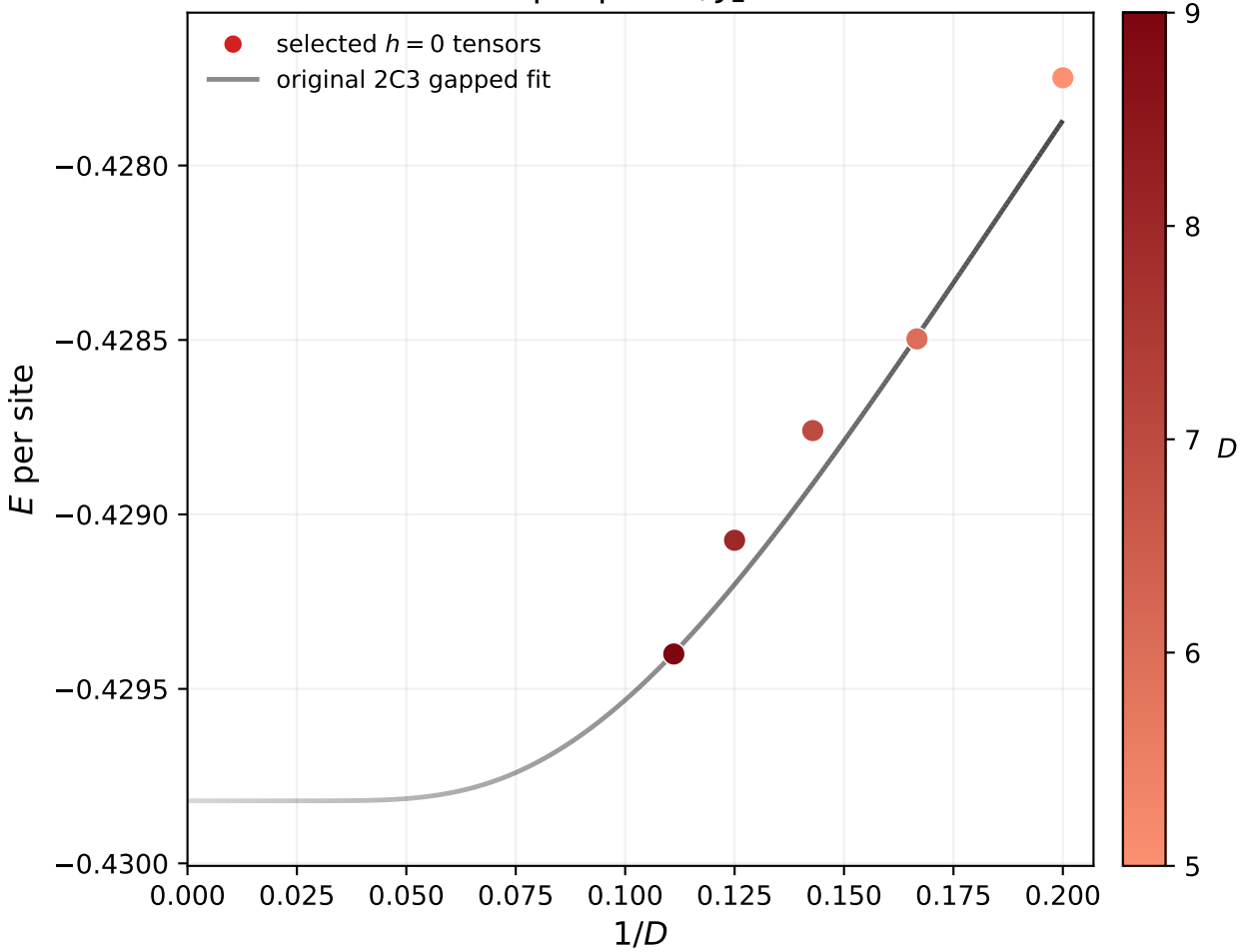
Dimer-plaquette, J_2 = 0.28
