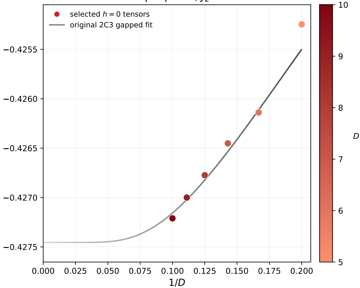
Dimer-plaquette, J_2 = 0.29
