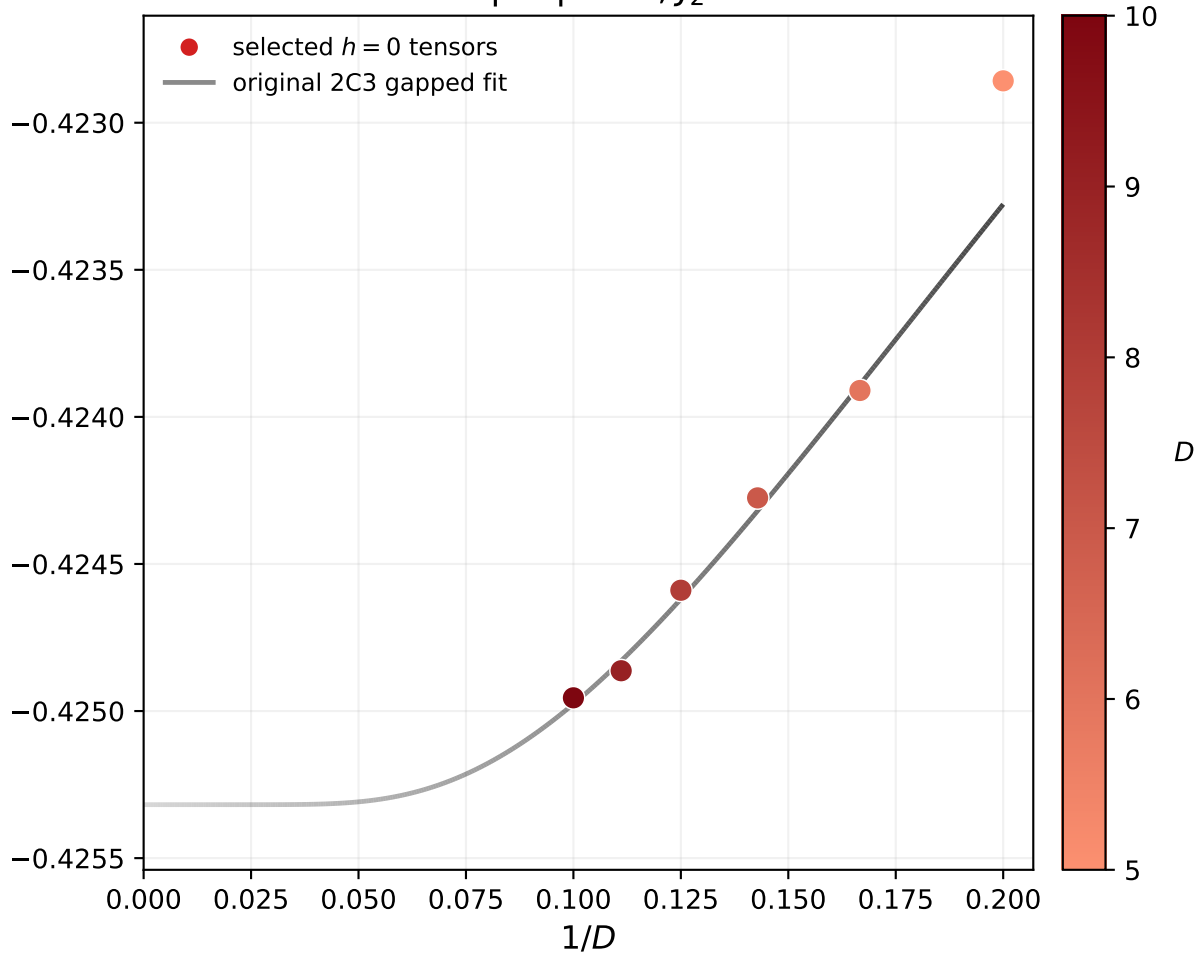
Dimer-plaquette, J_2 = 0.3
