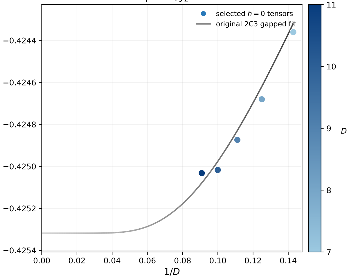
Plaquette, J_2 = 0.3
