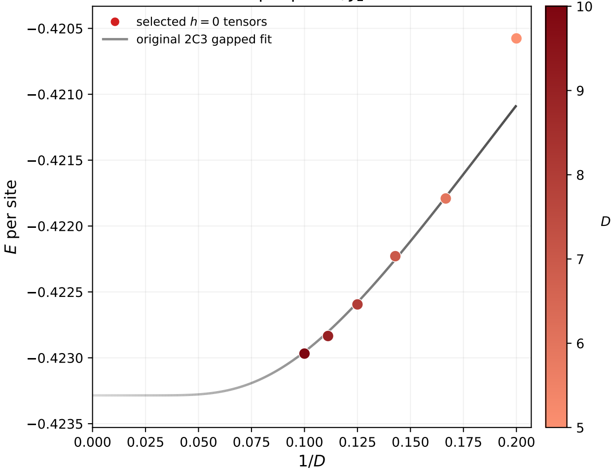
Dimer-plaquette, J_2 = 0.31
