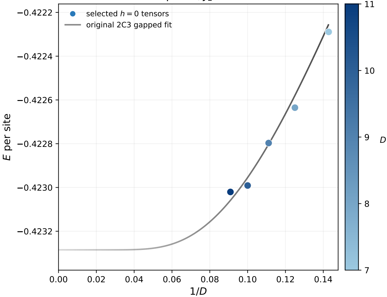
Plaquette, J_2 = 0.31
