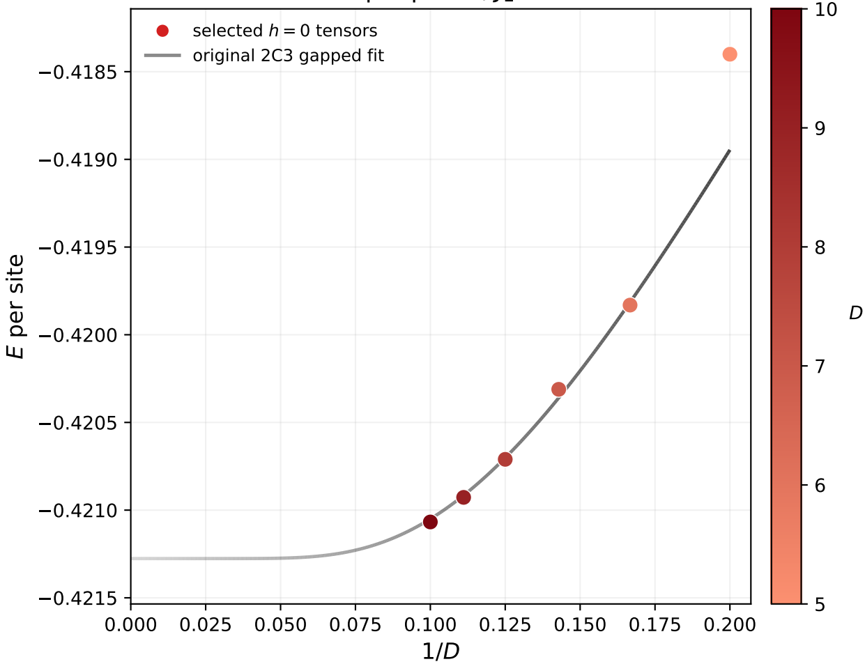
Dimer-plaquette, J_2 = 0.32
