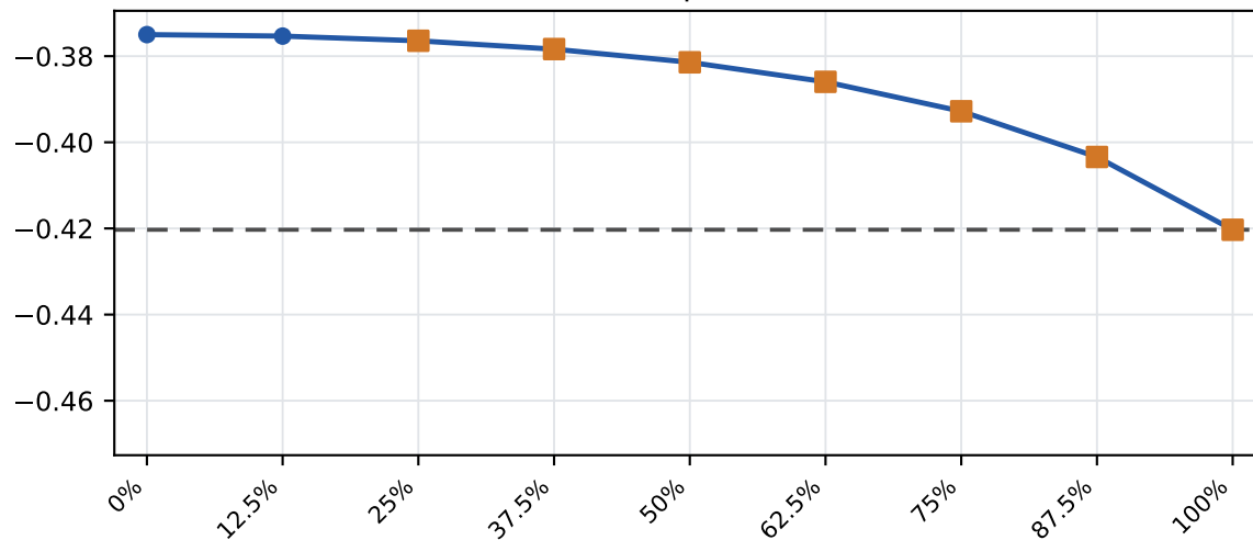
D = 7 | Dimer
