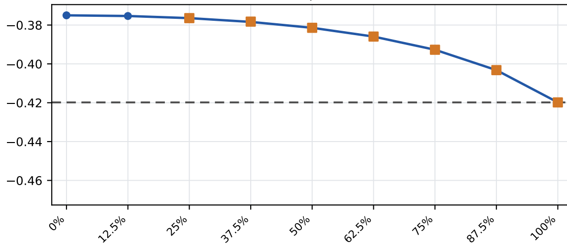
D = 6 | Dimer
