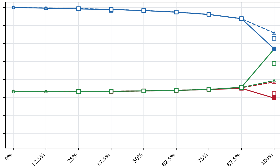
Plaquette
