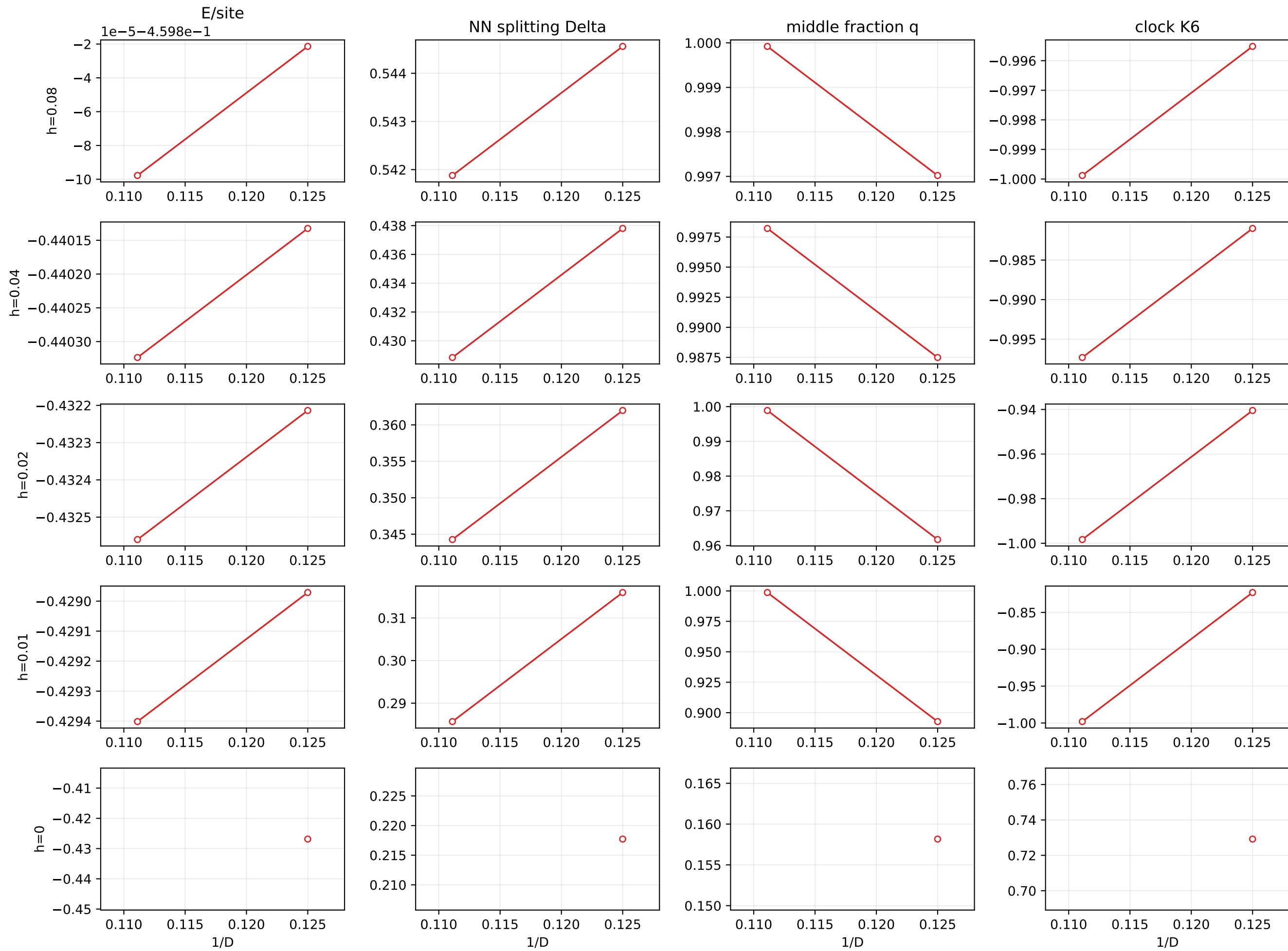
Izar replica 1, J2=0.29, dimer source: fixed-h trends; only h=0 energy is unbiased
