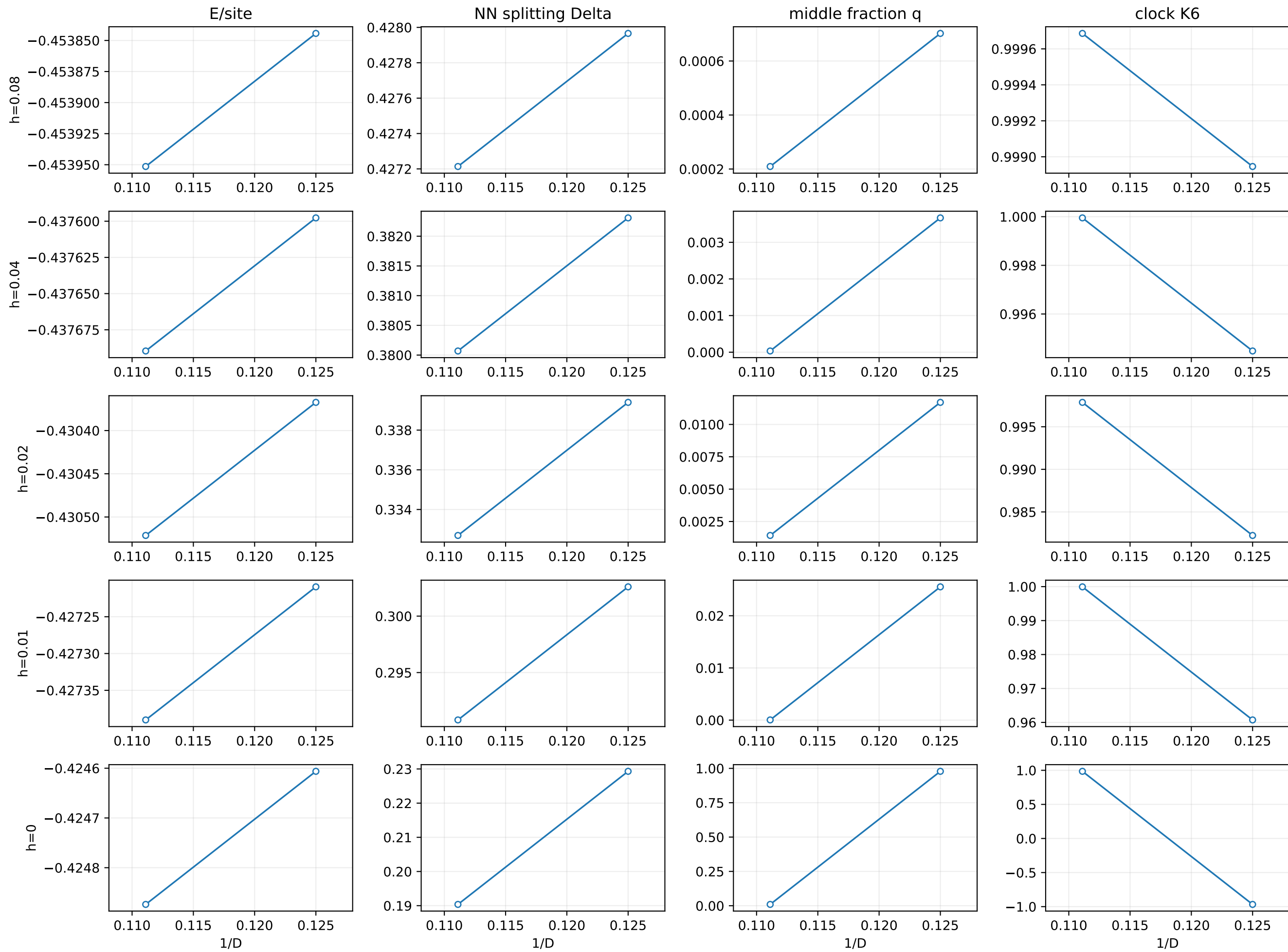
Izar replica 1, J2=0.30, plaquette source: fixed-h trends; only h=0 energy is unbiased
