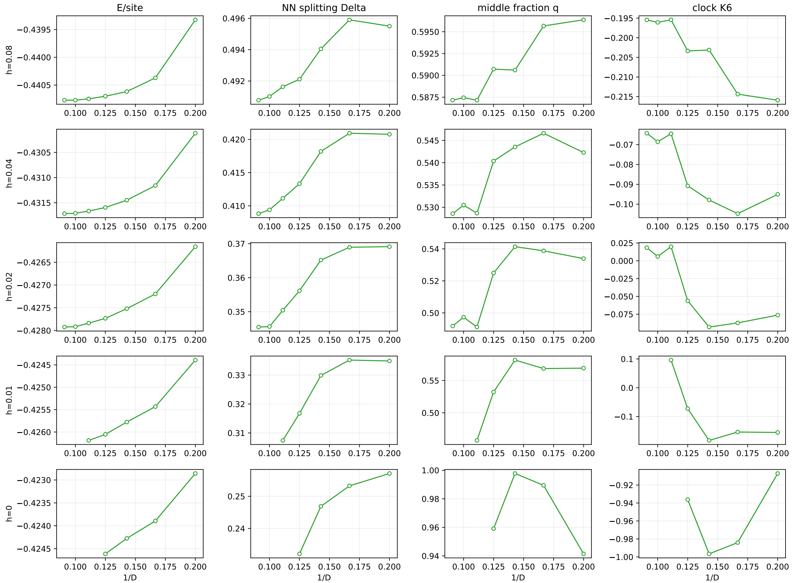
Kuma replica 1, J2=0.30, rank-split source: fixed-h trends; only h=0 energy is unbiased
