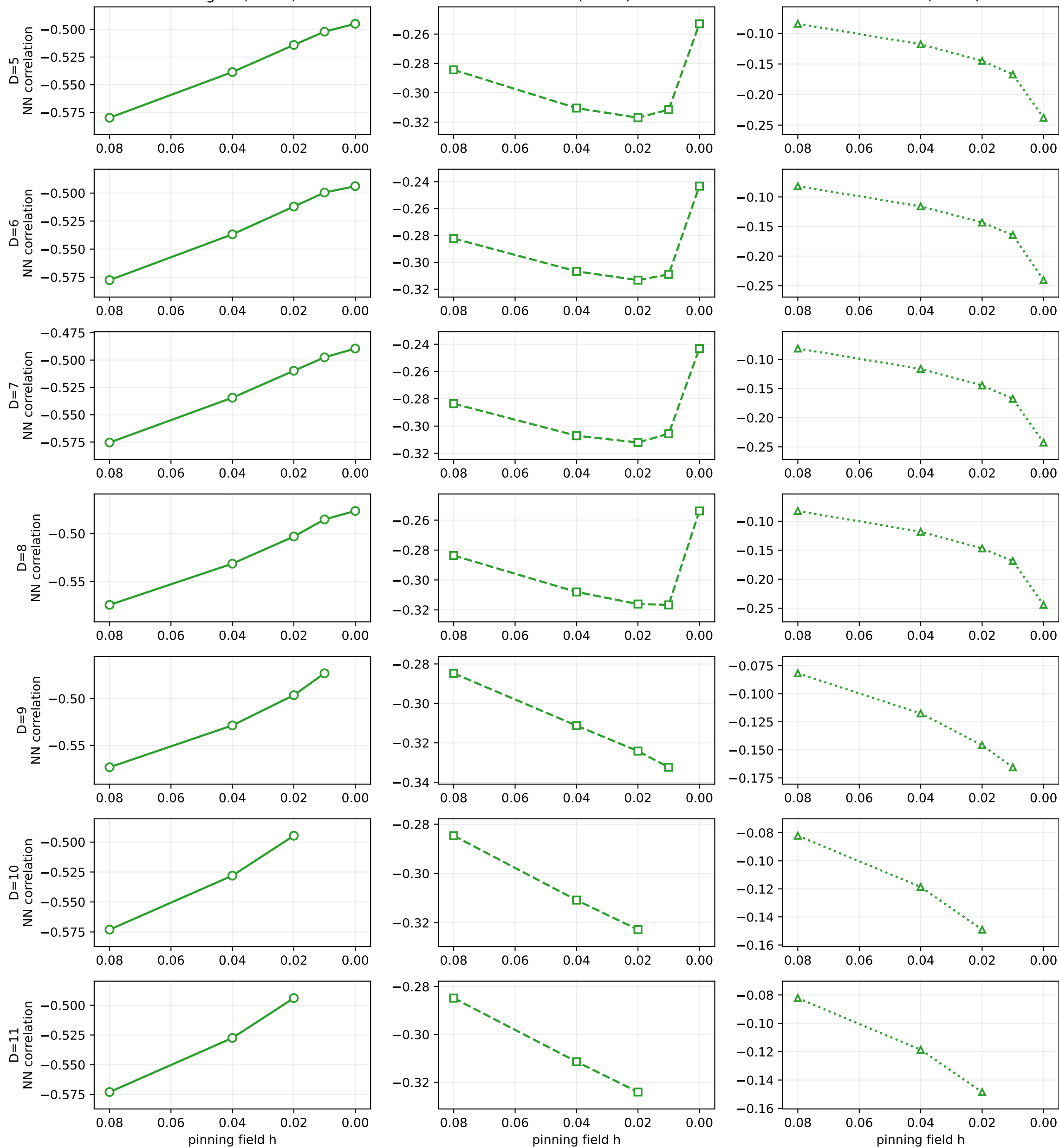
Kuma replica 1, J_2=0.30 , rank-split source: one rank per panel (independent vertical scales)
