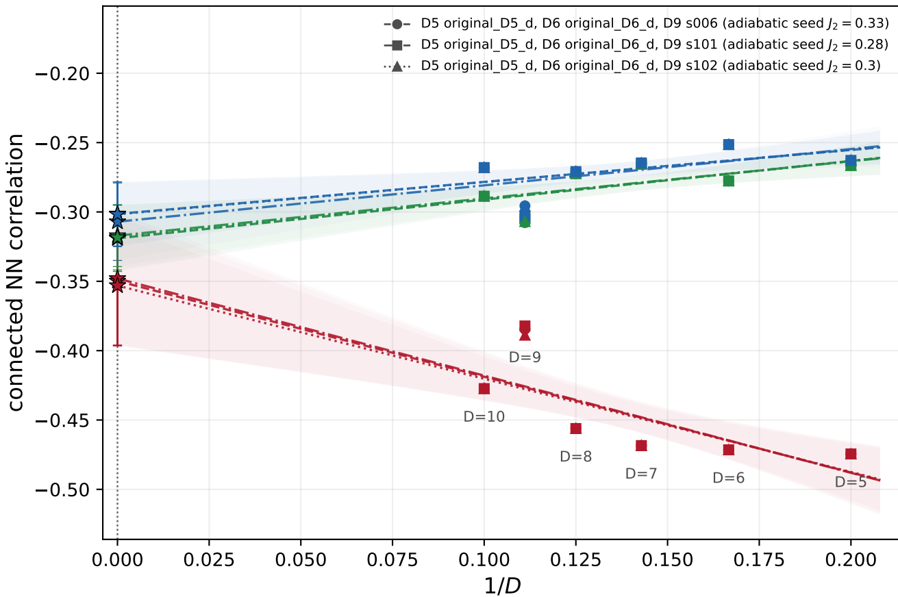
Dimer-plaquette sector, J_2 = 0.27
