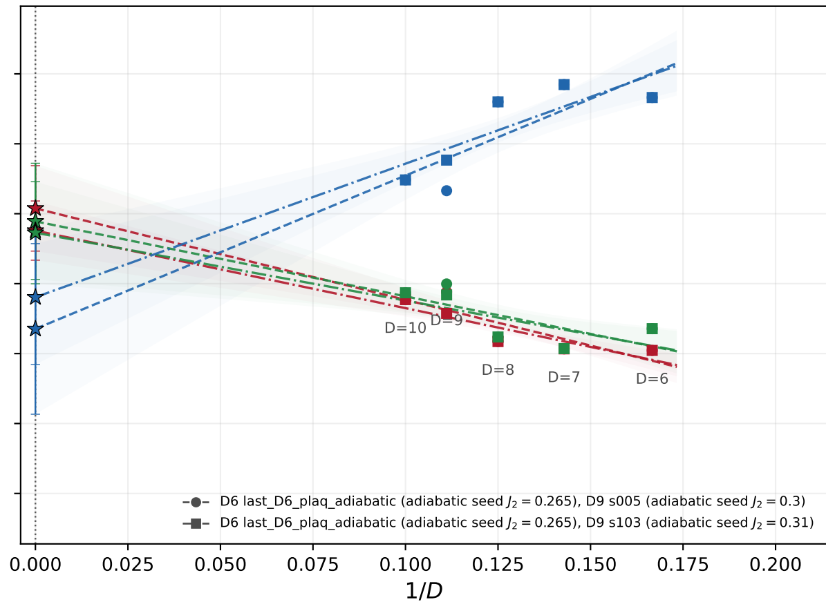
Plaquette sector, J_2 = 0.27
