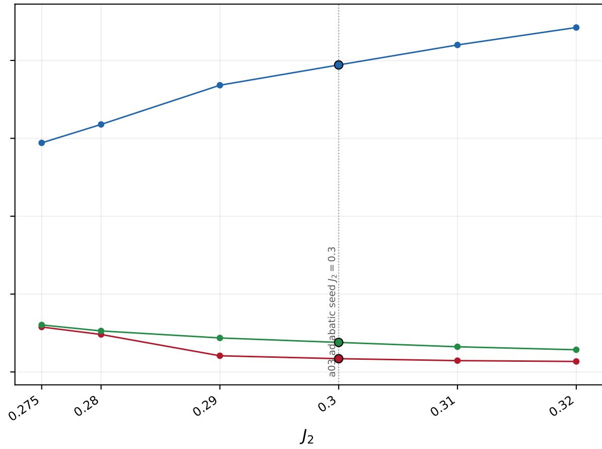
Plaquette sector, D = 11
