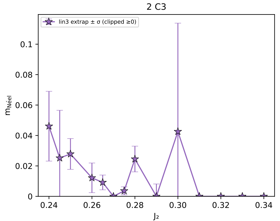
m_{\text{Néel}} vs J_2 — extrapolated \pm \sigma
