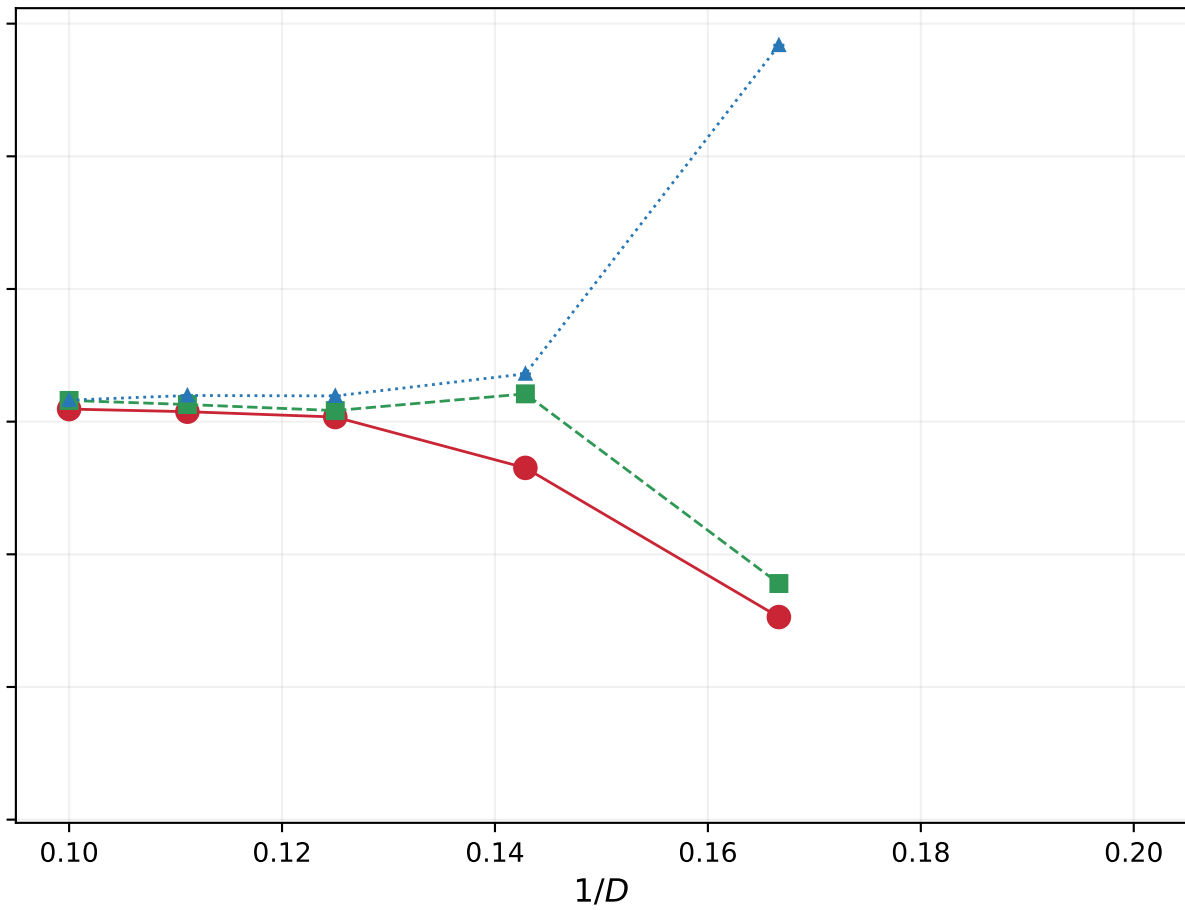
Plaquette sector, J_2 = 0.26
