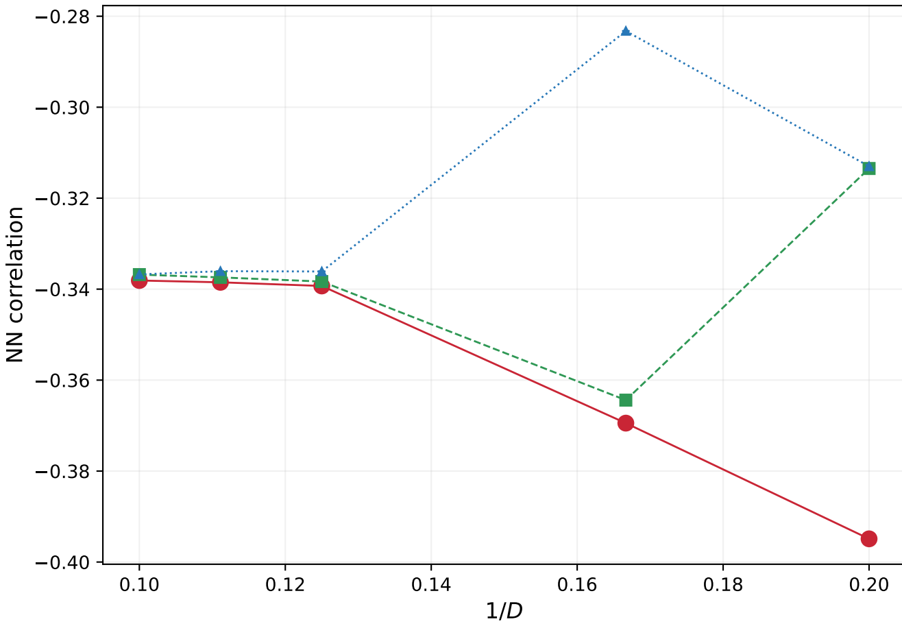
Dimer-plaquette sector, J_2 = 0.26
