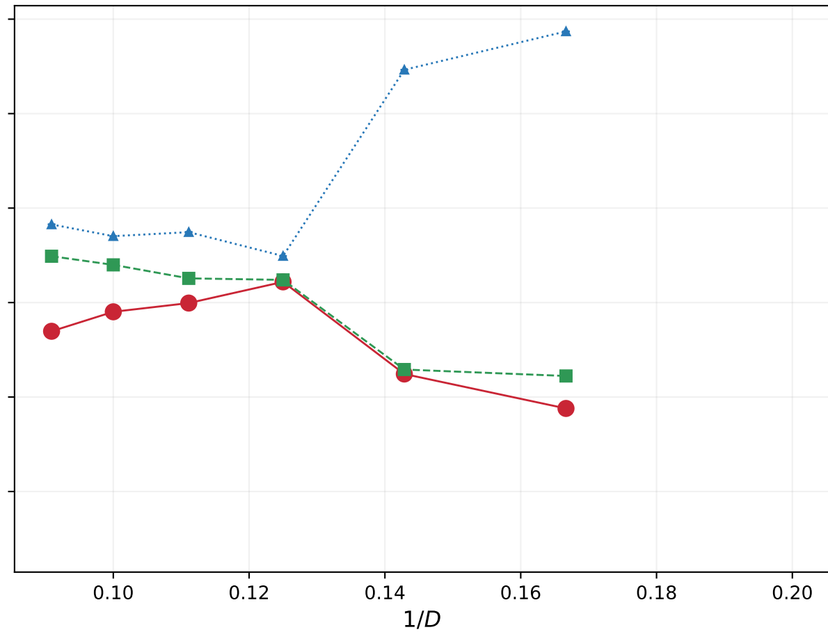
Plaquette sector, J_2 = 0.275
