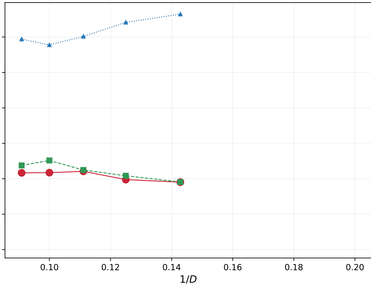
Plaquette sector, J_2 = 0.3
