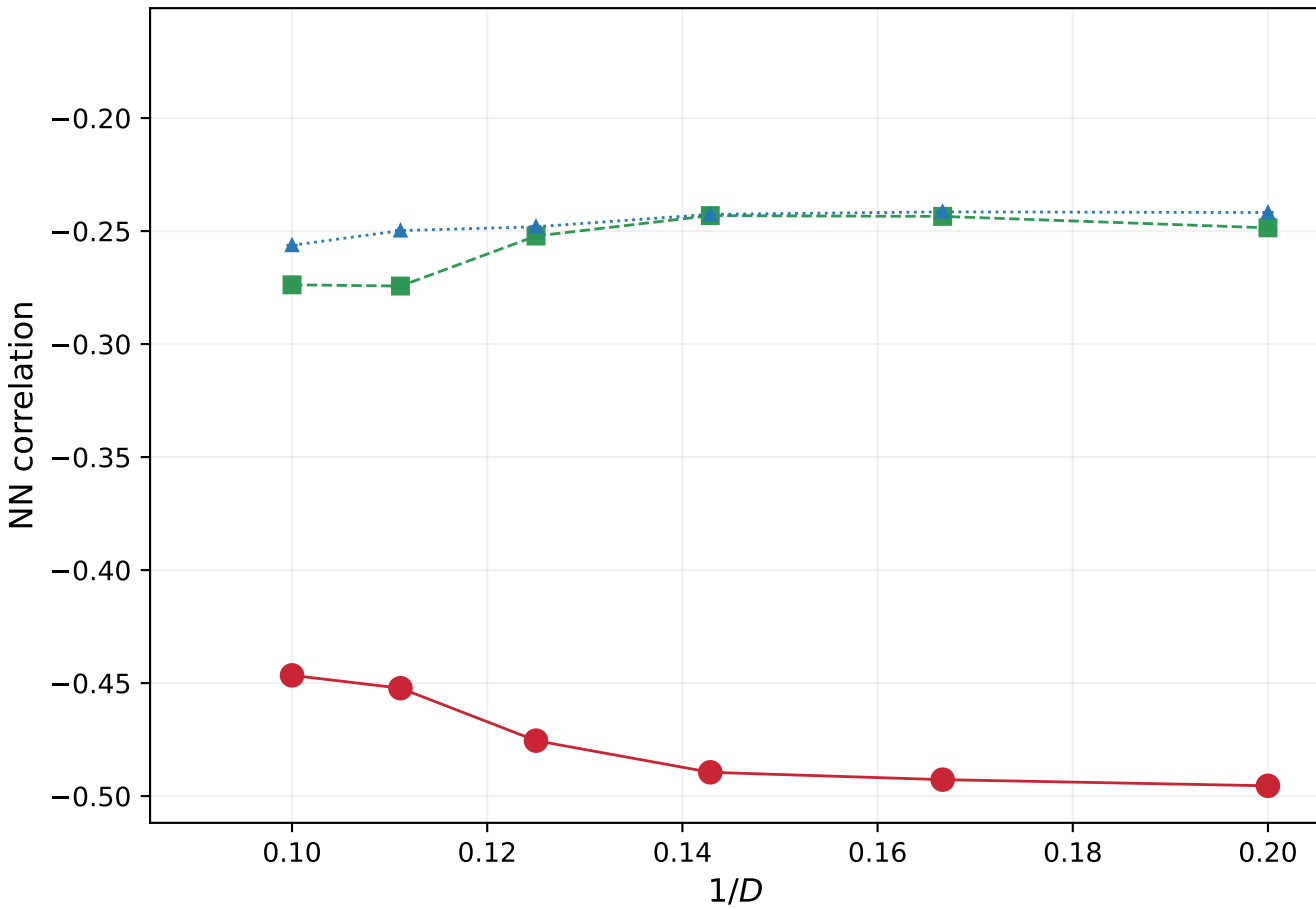
Dimer-plaquette sector, J_2 = 0.3
