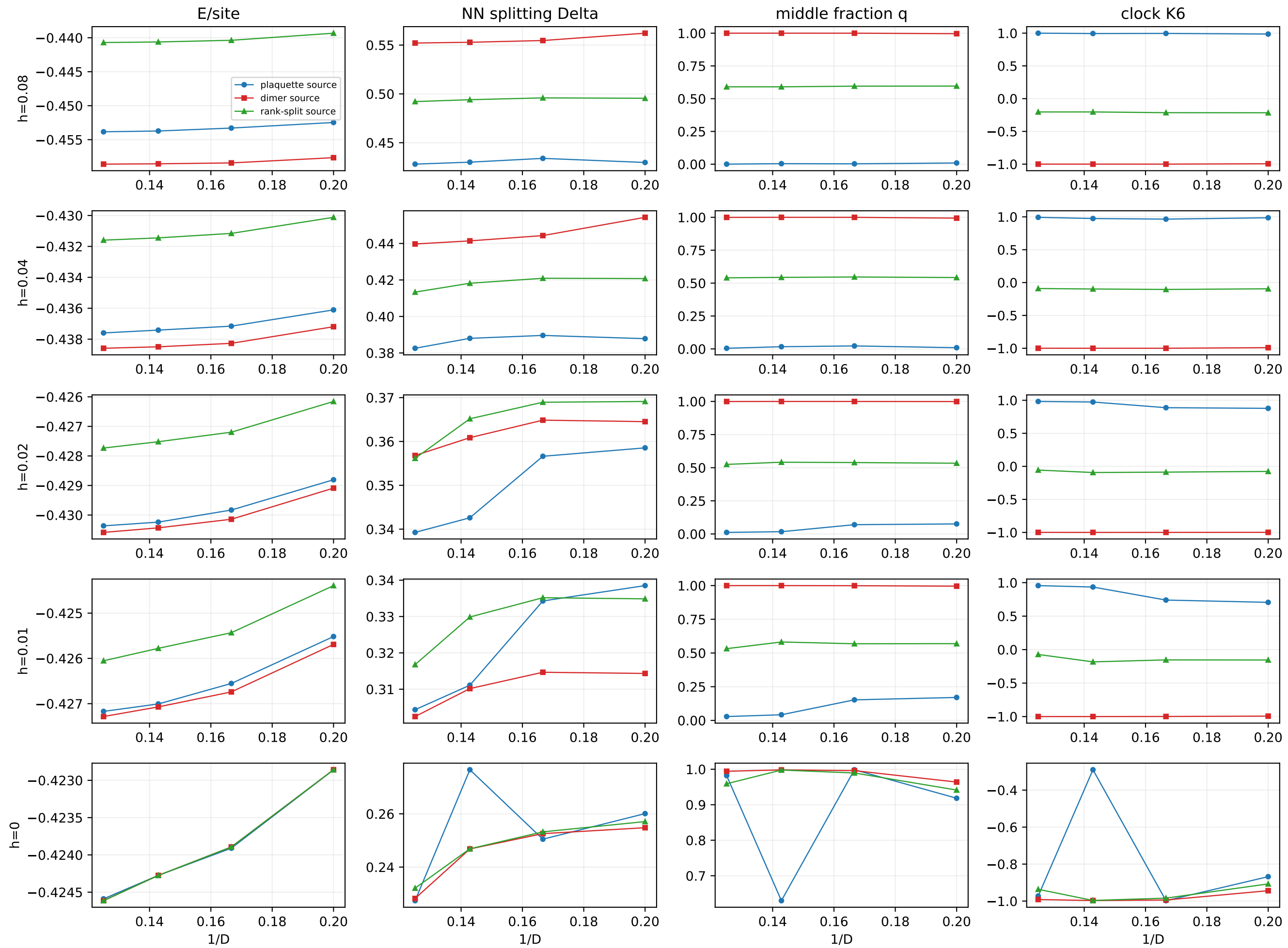
Fixed-h trends; only h=0 energy curves share the same Hamiltonian
