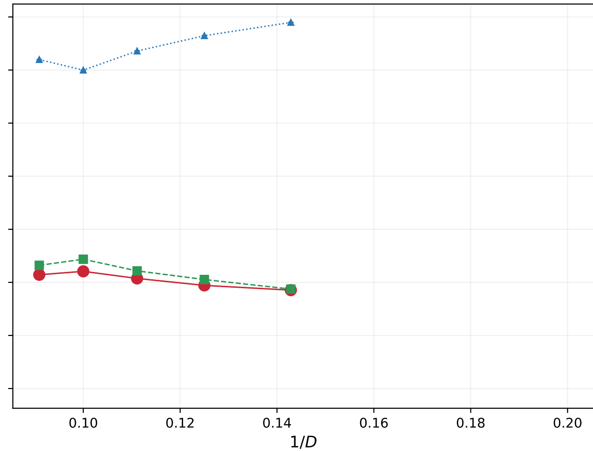
Plaquette sector, J_2 = 0.31
