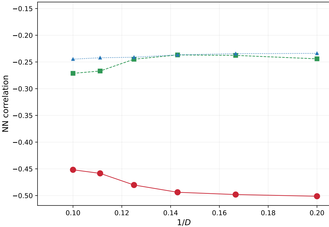
Dimer-plaquette sector, J_2 = 0.31
