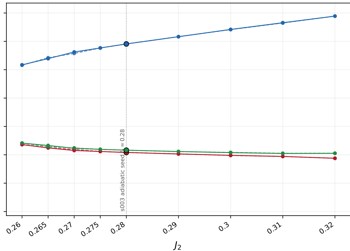
Plaquette sector, D = 8
