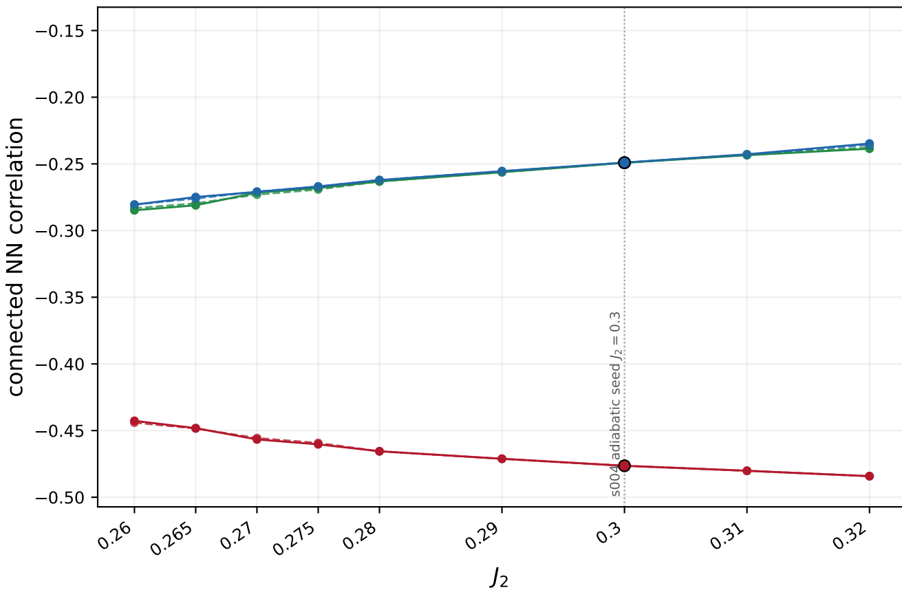
Dimer-plaquette sector, D = 8
