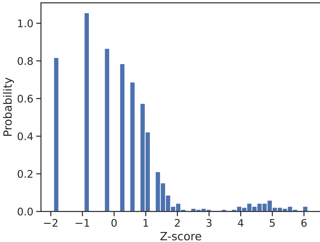
MUT Z-scores
