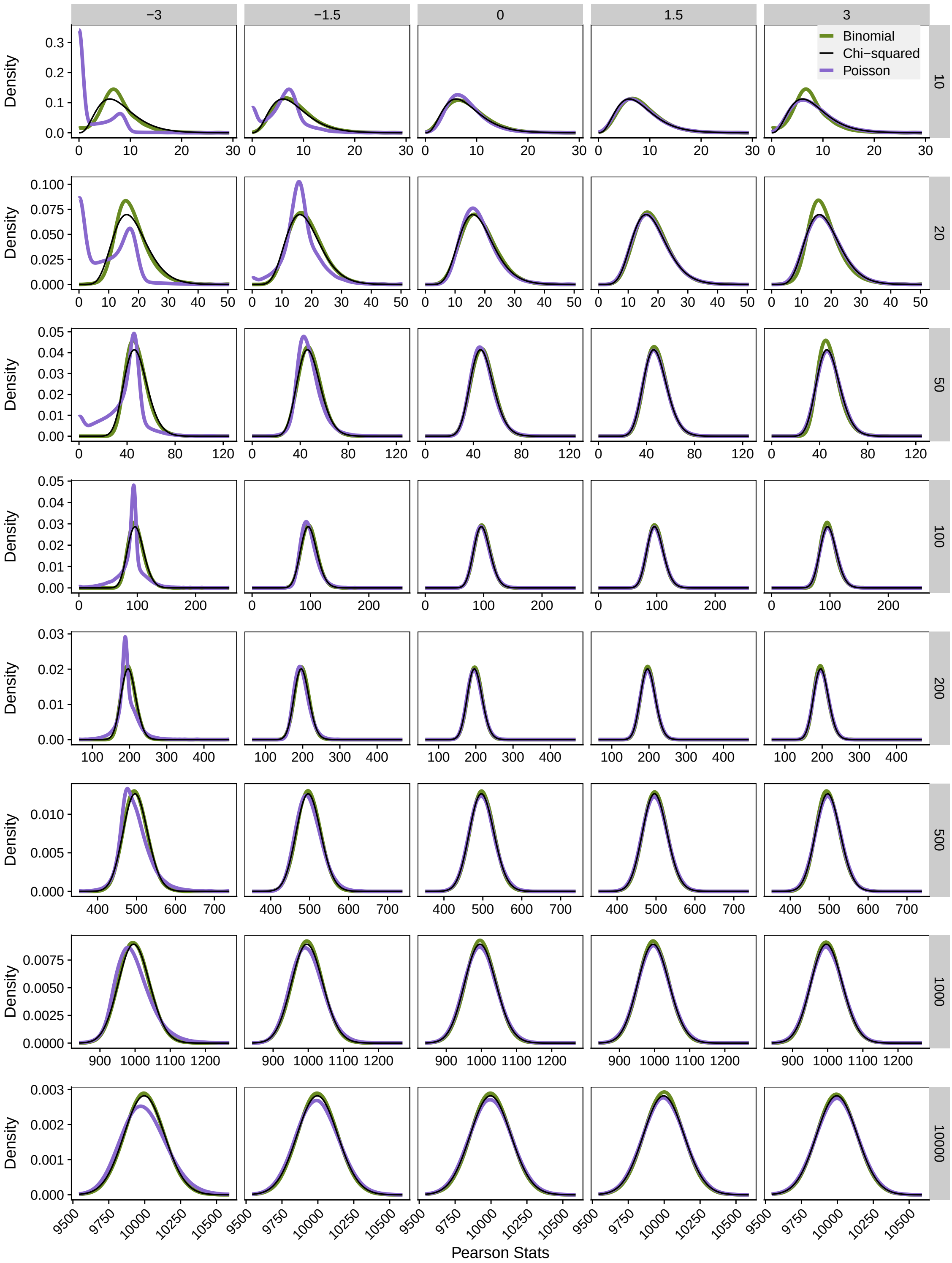
Pearson statistics X Chi-squared distribution
