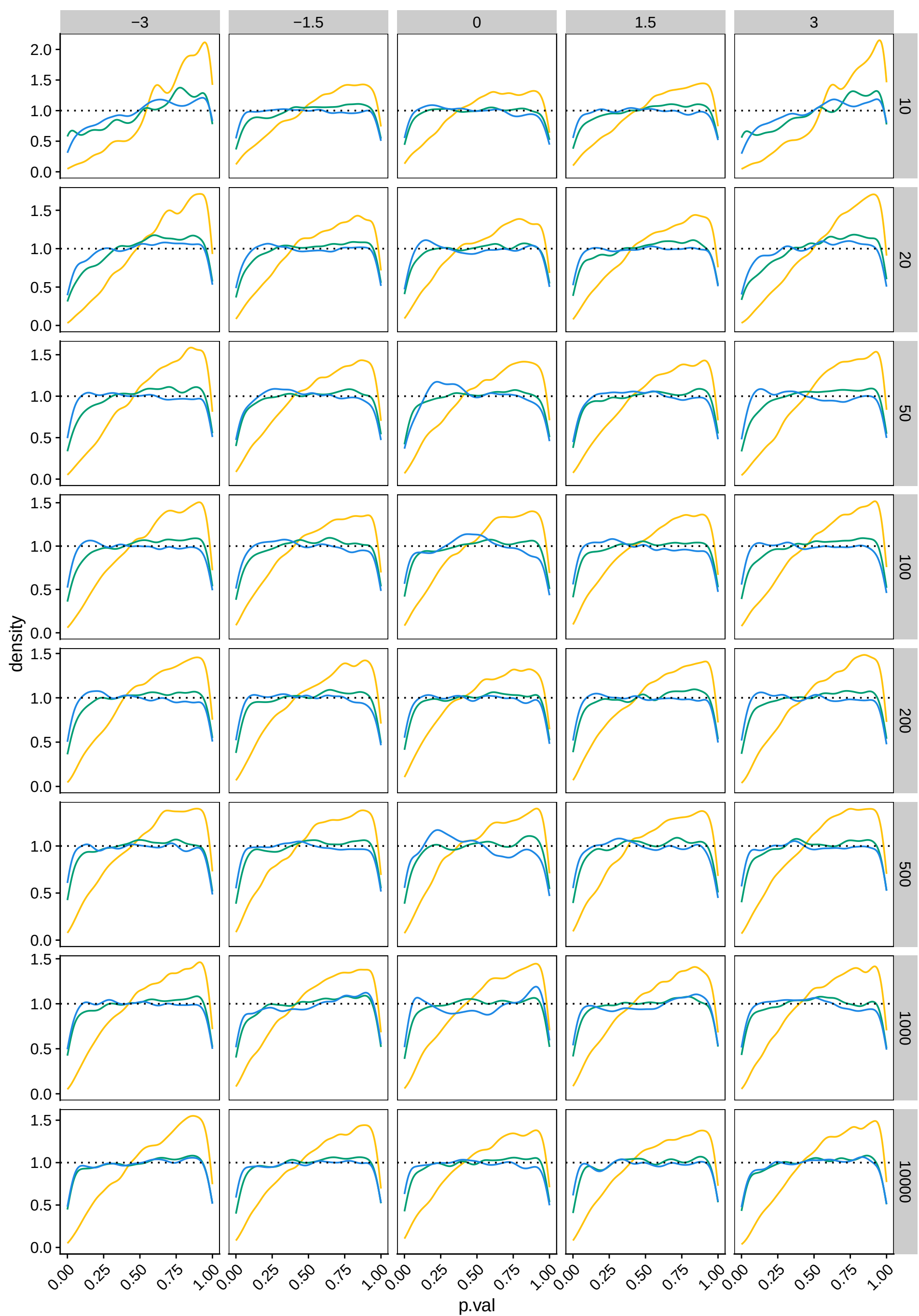
Binomial: distribution P-values
