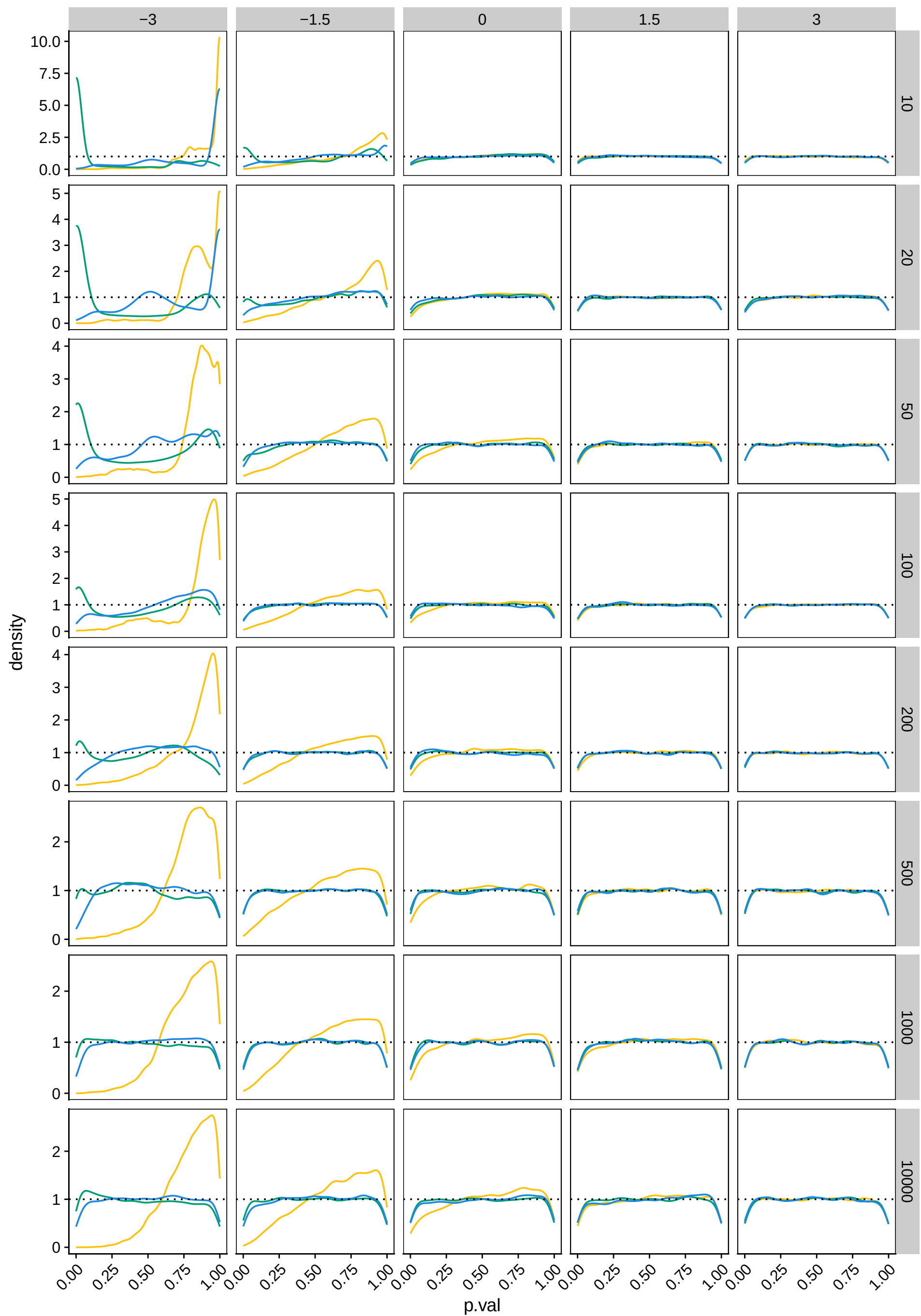
Poisson: distribution P-values
