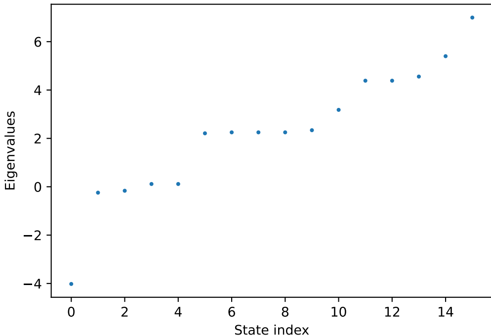
(2×2) Lattice, Cutoff 1, Number of States 16
