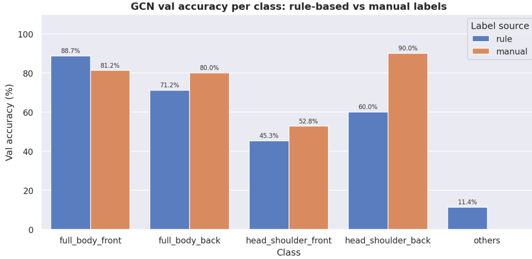
Figure 4: Per-class GCN validation accuracy when trained on rule-based vs. manually annotated labels.
