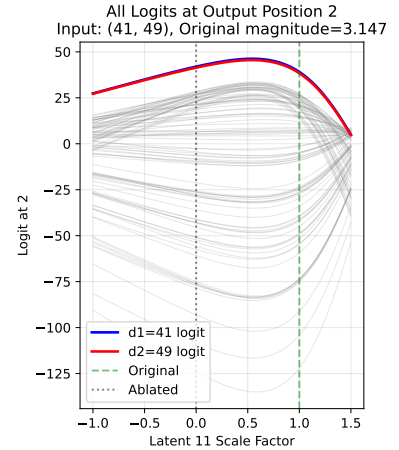
Figure 13. Moreover, in the same SAE, if latent 55's activation magnitude is scaled by a factor of 1.1, then we can now scale latent 11 by factor p \in [0.03, 1.45] to swap the outputs, which was not possible without scaling latent 55. This suggests that some graded activation demonstrations are only possible when multiple active latents are scaled simultaneously.
