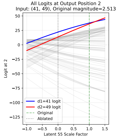
Figure 12. However, in the same SAE, latent 55 co-activates with latent 11 for input (41, 49) and can be scaled by factor p \in [1.07, 1.18] to cause the model to output (49, 41) instead.
