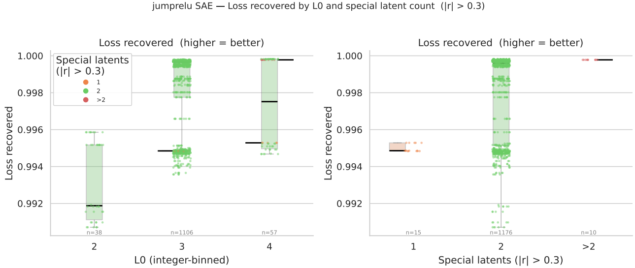
Figure 14. These strip plots show how the number of special latents (identified by the latent activation’s correlation with \Delta\alpha using threshold |r| > 0.3 , as in Section 3.1) differs across all JumpReLU SAEs from the sweep in Table 4.
