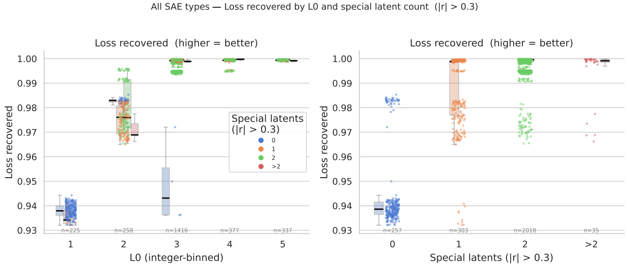
Figure 12. These strip plots show how the number of special latents (identified by the latent activation’s correlation with \Delta\alpha using threshold |r| > 0.3 , as in Section 3.1) differs across all 2,613 trained SAEs from the sweep in Table 4. Left: A large majority of the SAEs achieve L0 \approx 3 . However, only those with special latents achieve high performance. Right: SAEs with no special latents tend to perform much worse than those with them. Most SAEs learn two special latents.
