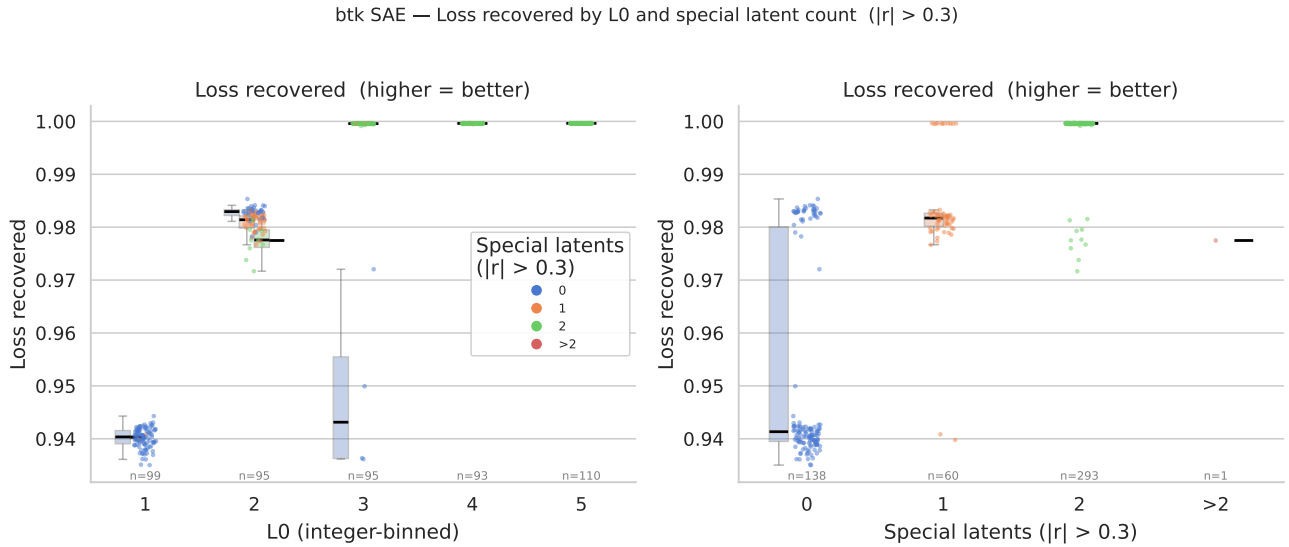
Figure 13. These strip plots show how the number of special latents (identified by the latent activation’s correlation with \Delta\alpha using threshold |r| > 0.3 , as in Section 3.1) differs across all BatchTopK SAEs from the sweep in Table 4.
