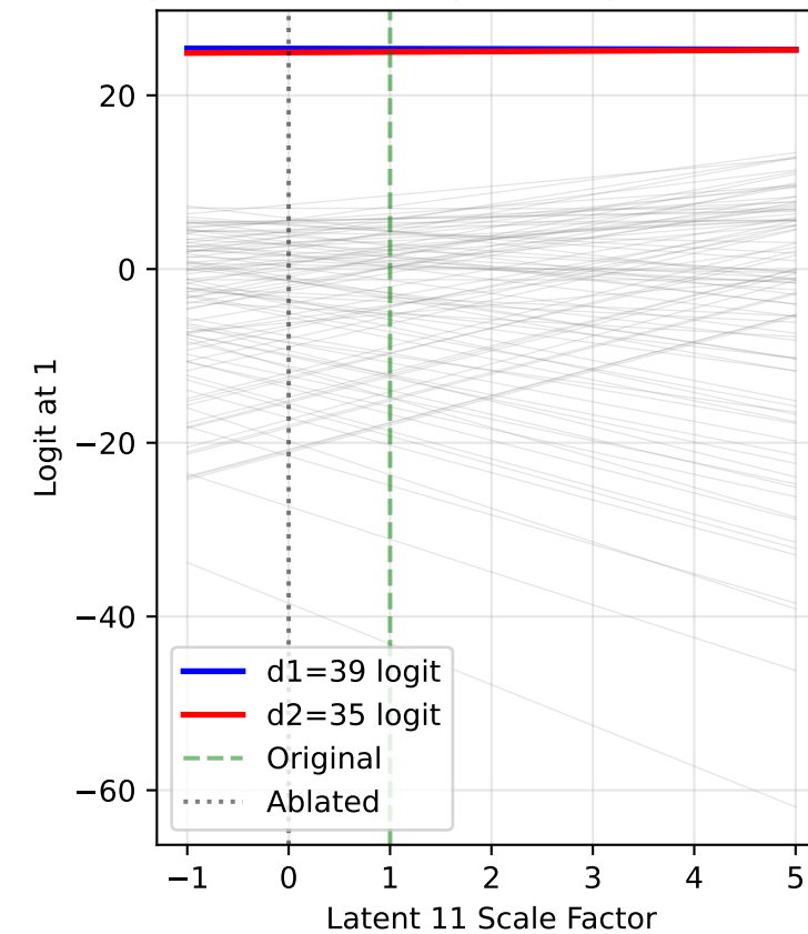
All Logits at Output Position 1 Input: (39, 35), Original magnitude=0.416
