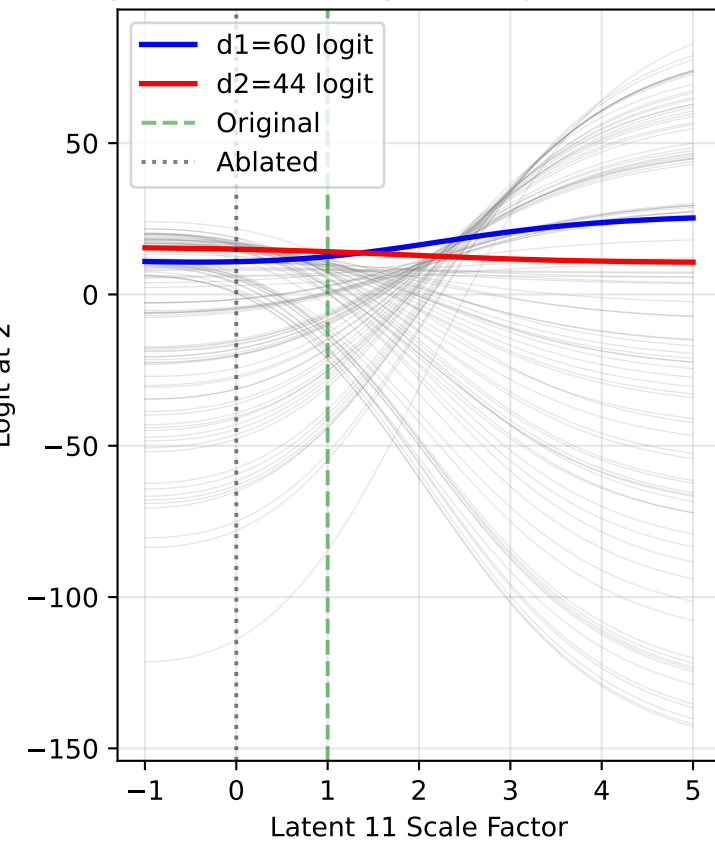
All Logits at Output Position 2 Input: (60, 44), Original magnitude=1.026
