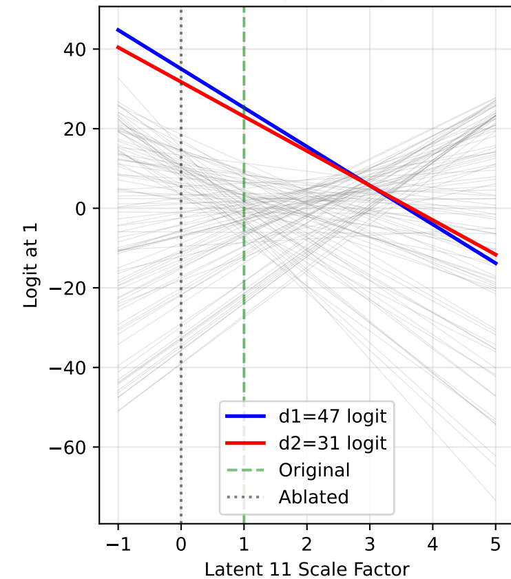
All Logits at Output Position 1 Input: (47, 31), Original magnitude=1.571
