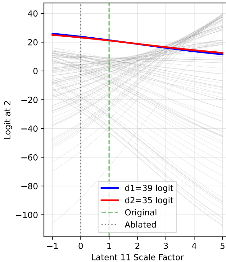
All Logits at Output Position 2 Input: (39, 35), Original magnitude=0.416
