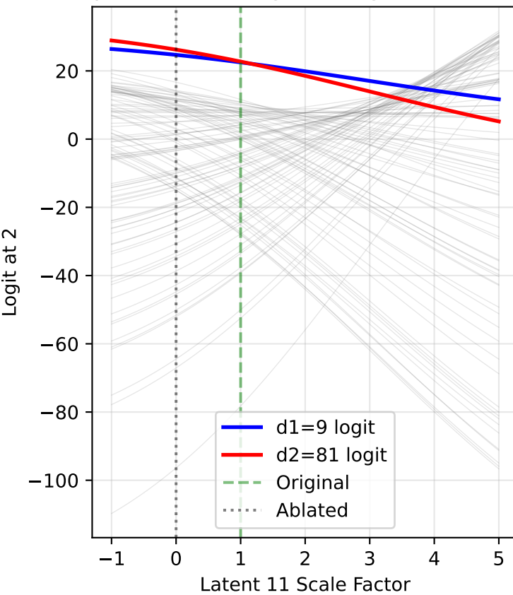
All Logits at Output Position 2 Input: (9, 81), Original magnitude=0.424
