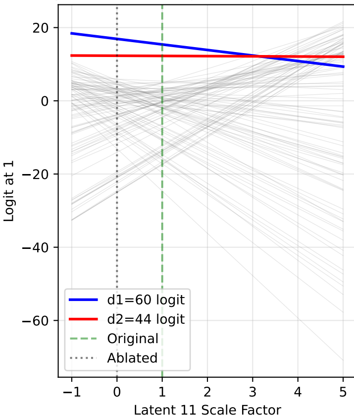
All Logits at Output Position 1 Input: (60, 44), Original magnitude=1.026
