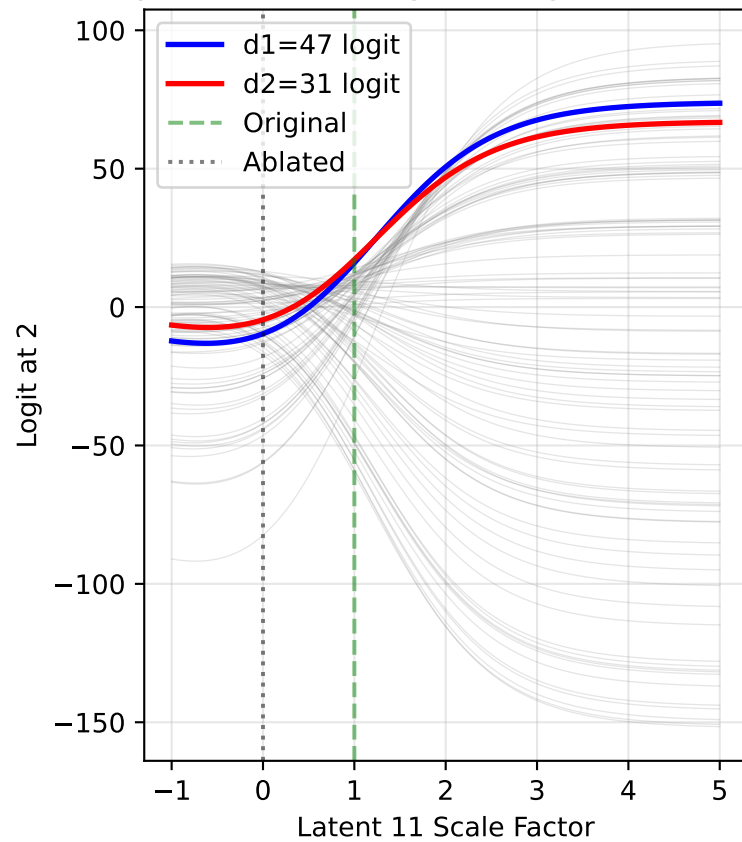
All Logits at Output Position 2 Input: (47, 31), Original magnitude=1.571
