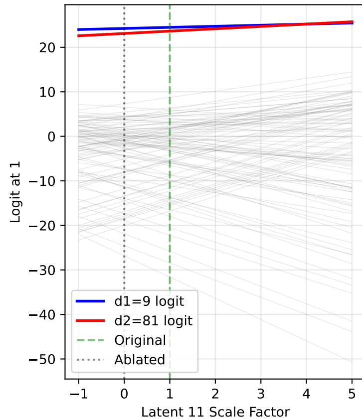
All Logits at Output Position 1 Input: (9, 81), Original magnitude=0.424
