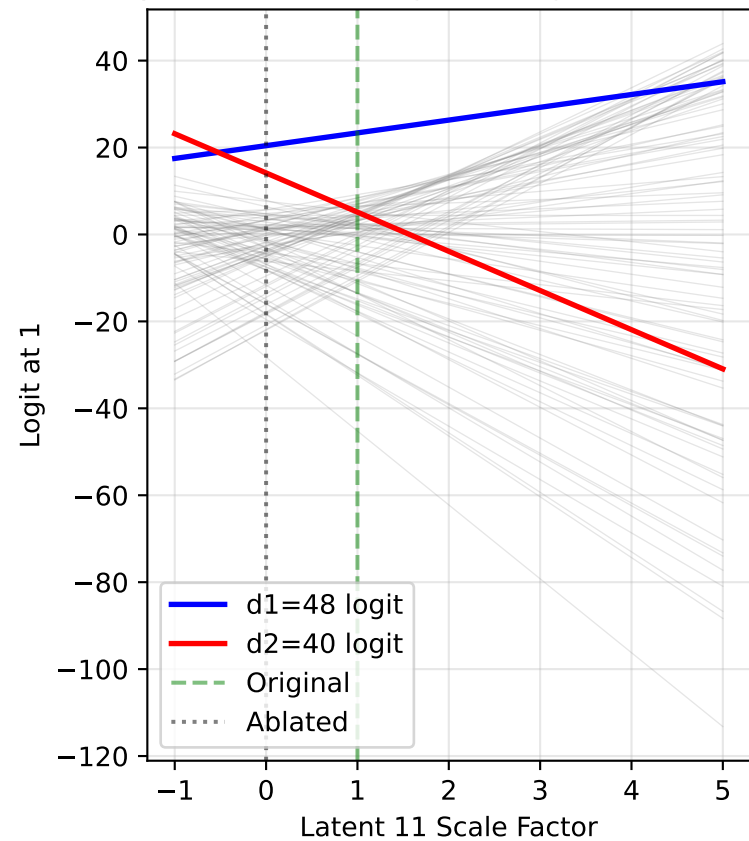
All Logits at Output Position 1 Input: (48, 40), Original magnitude=1.510
