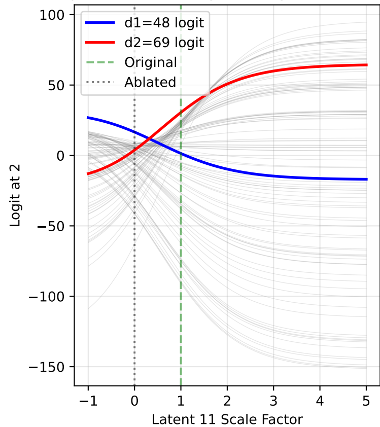
All Logits at Output Position 2 Input: (48, 69), Original magnitude=1.243
