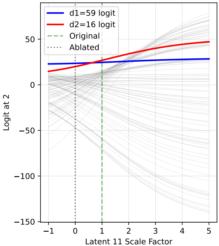
All Logits at Output Position 2 Input: (59, 16), Original magnitude=0.640
