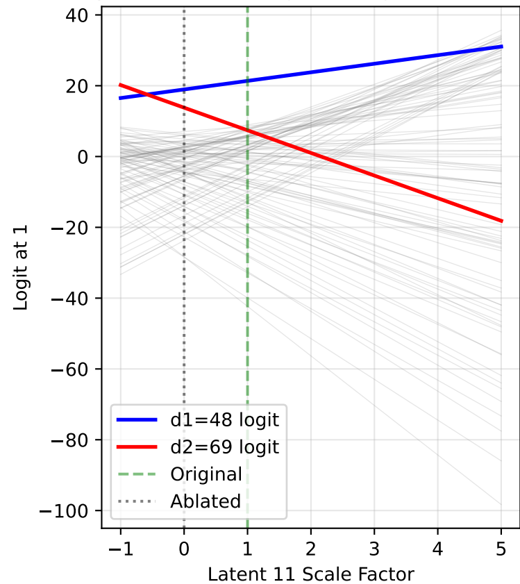
All Logits at Output Position 1 Input: (48, 69), Original magnitude=1.243
