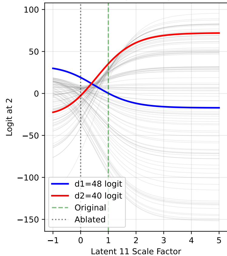
All Logits at Output Position 2 Input: (48, 40), Original magnitude=1.510
