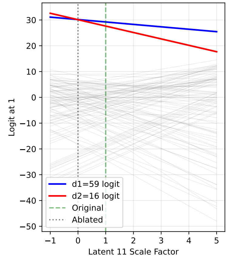
All Logits at Output Position 1 Input: (59, 16), Original magnitude=0.640
