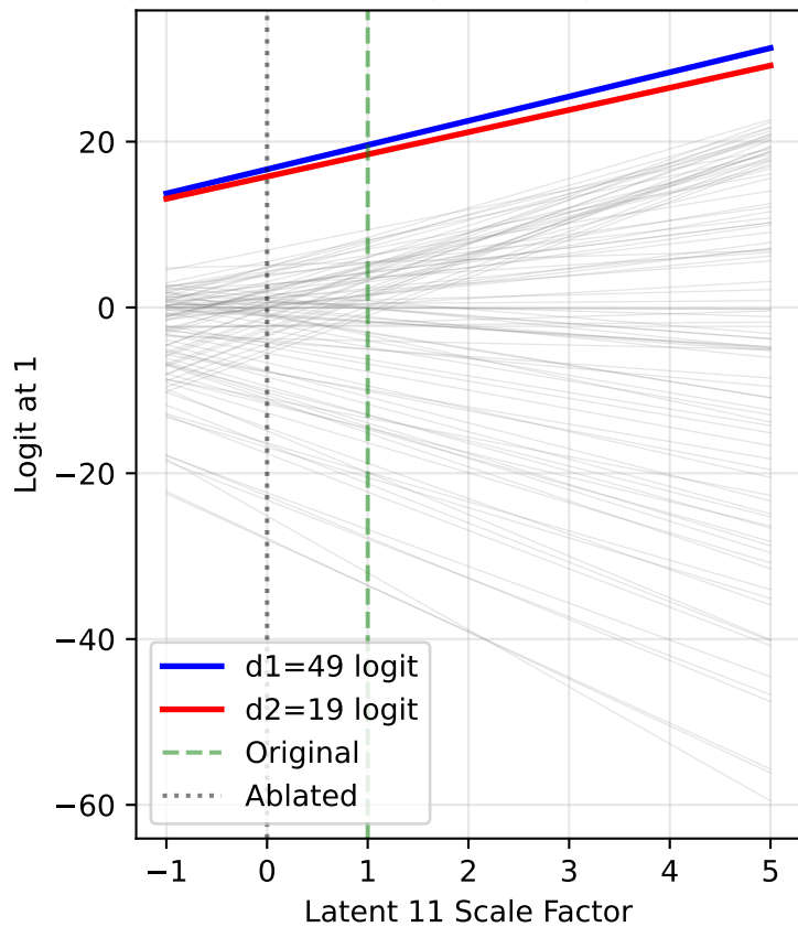
All Logits at Output Position 1 Input: (49, 19), Original magnitude=0.611
