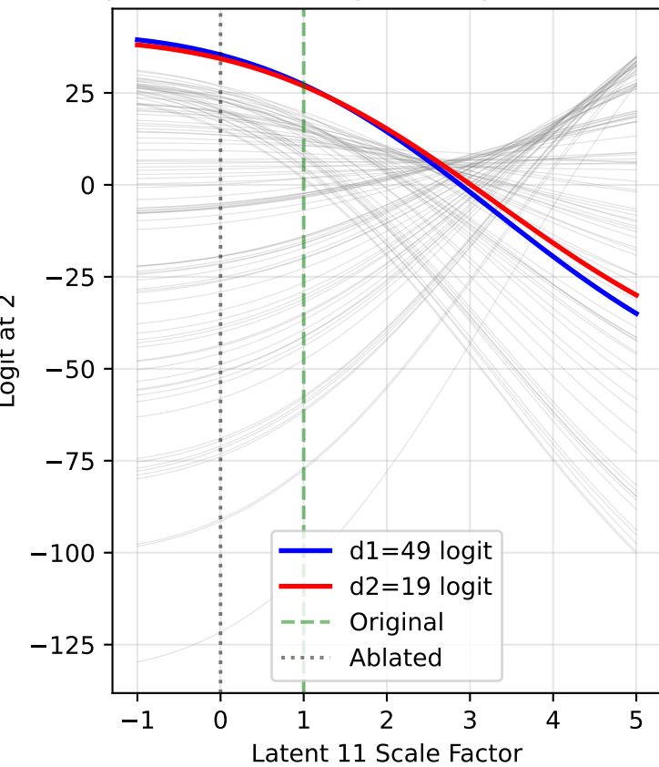
All Logits at Output Position 2 Input: (49, 19), Original magnitude=0.611
