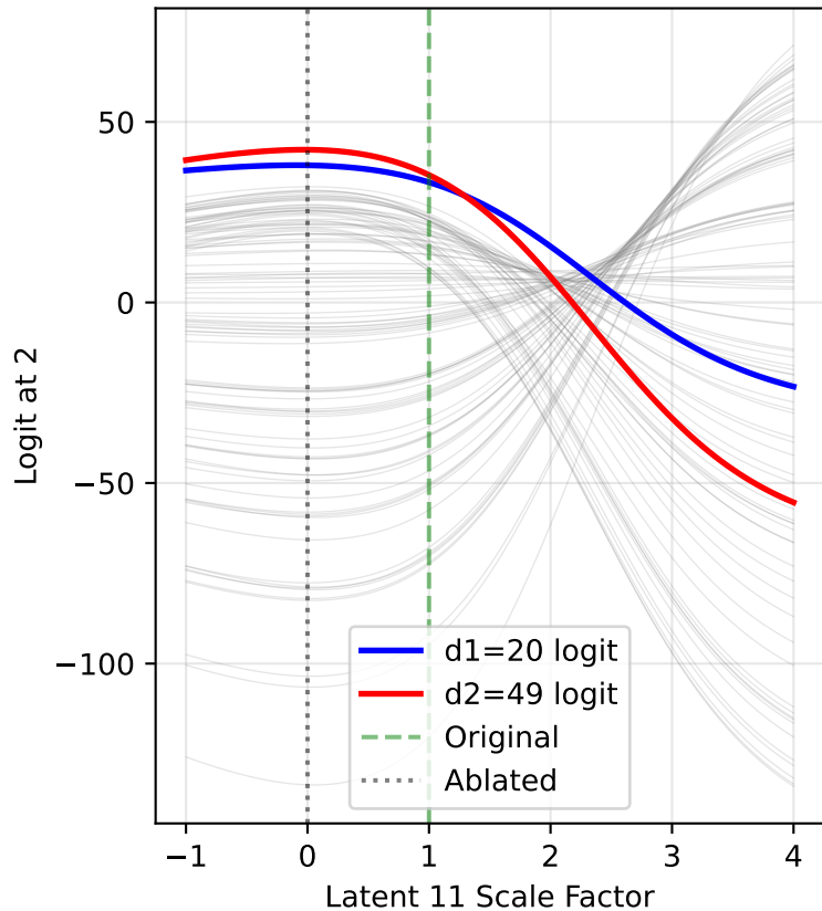
All Logits at Output Position 2 Input: (20, 49), Original magnitude=1.403
