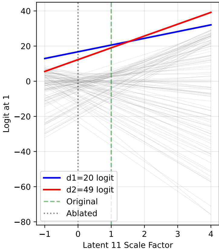
All Logits at Output Position 1 Input: (20, 49), Original magnitude=1.403
