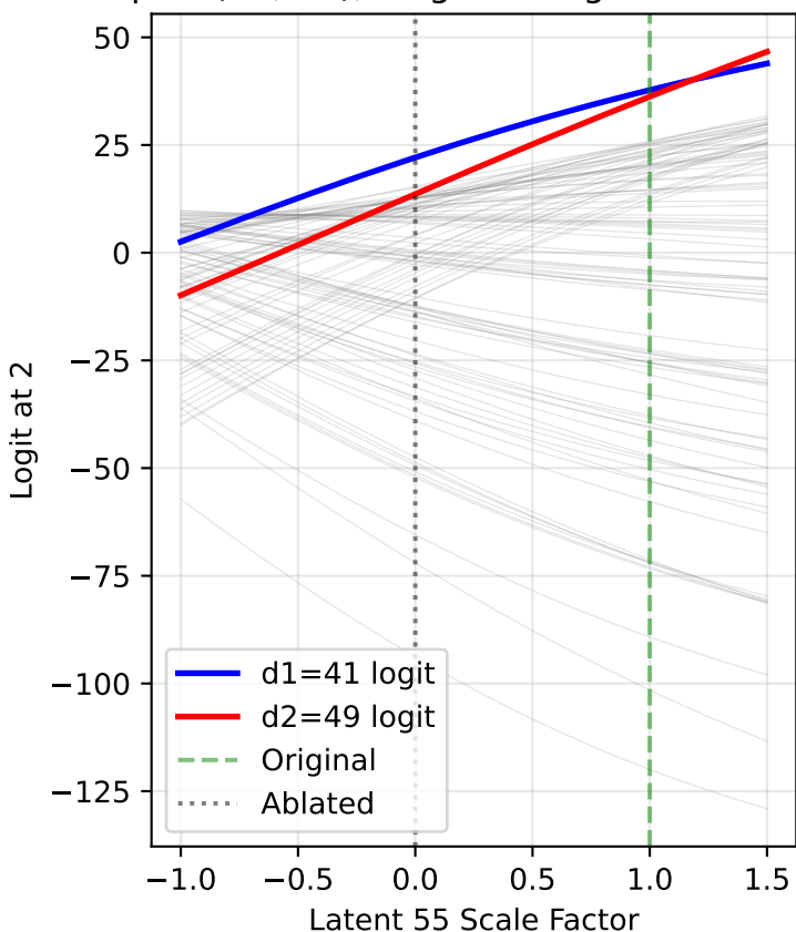
All Logits at Output Position 2 Input: (41, 49), Original magnitude=2.513
