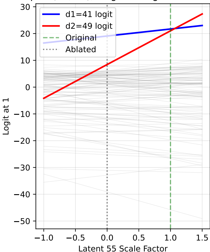
All Logits at Output Position 1 Input: (41, 49), Original magnitude=2.513
