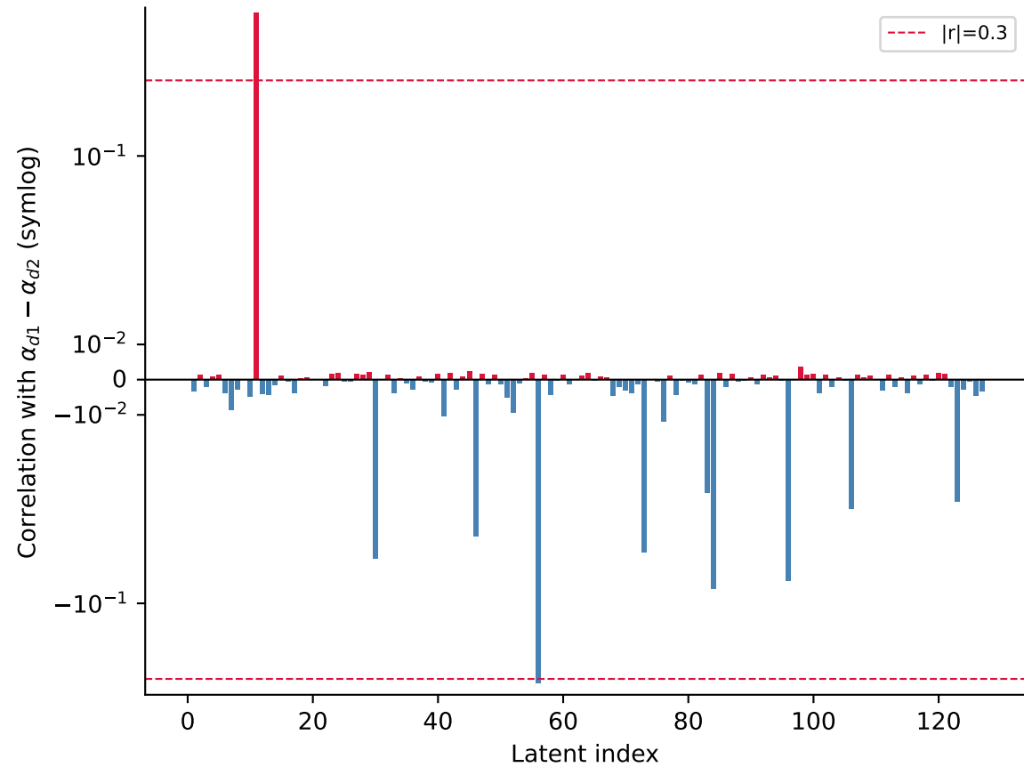
Latent- \Delta\alpha correlations
