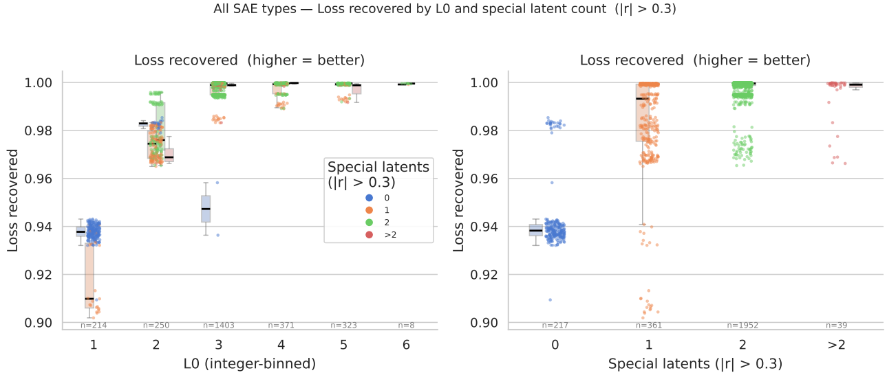
Figure 12. These strip plots show how the number of special latents (identified by the latent’s activation’s correlation with \Delta\alpha using threshold |r| > 0.3 , as in Section 3.1) differs across SAEs with different sparsities and performance. This includes all SAEs from the sweep in Table 4. Left: A large majority of the SAEs achieve L0 \approx 3 . However, only those with special latents achieve high performance. Right: SAEs with no special latents tend to perform much worse than those with them. Most SAEs learn two special latents.
