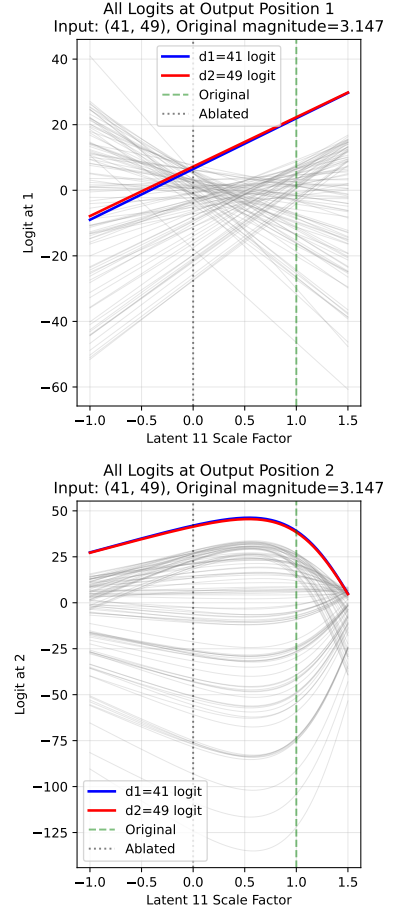
Figure 14. Moreover, in the same SAE, if latent 55's activation magnitude is scaled by a factor of 1.1, then we can now scale latent 11 by factor p \in [0.03, 1.45] to swap the outputs, which was not possible without scaling latent 55. This suggests that some graded activation demonstrations are only possible when multiple active latents are scaled simultaneously.
