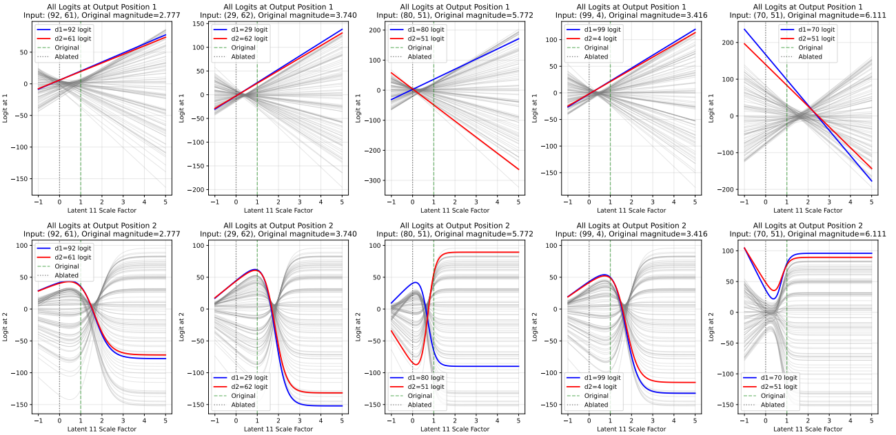
Figure 10. For 1.6% of inputs, the logit for the symbol at d_2 is always dominant at o_2 in the observed latent scale range (in the BatchTopK SAE from Section ??), so there is no scale where the symbol at d_1 is predicted instead.
