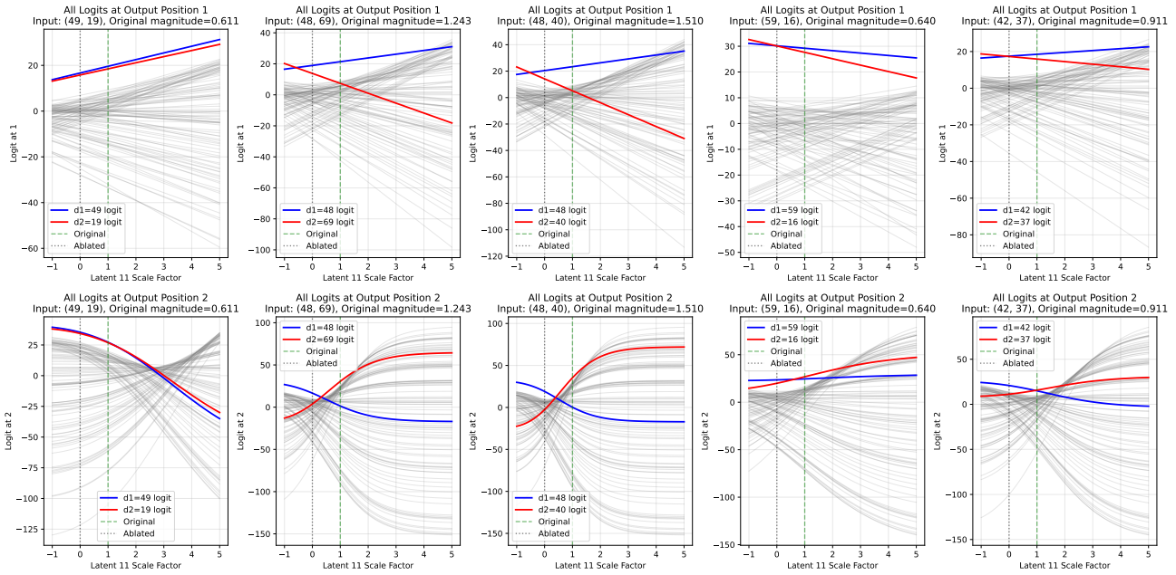
Figure 8. For 9.2% of inputs, latent 11 (in the BatchTopK SAE from Section ??) must be negatively scaled to swap the predicted symbol at one of the output positions.
