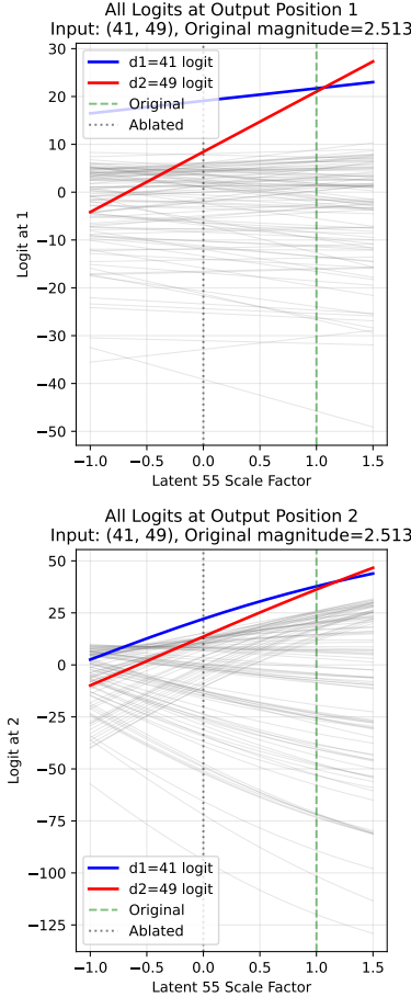
Figure 13. However, in the same SAE, latent 55 co-activates with latent 11 for input (41, 49) and can be scaled by factor p \in [1.07, 1.18] to cause the model to output (49, 41) instead.
