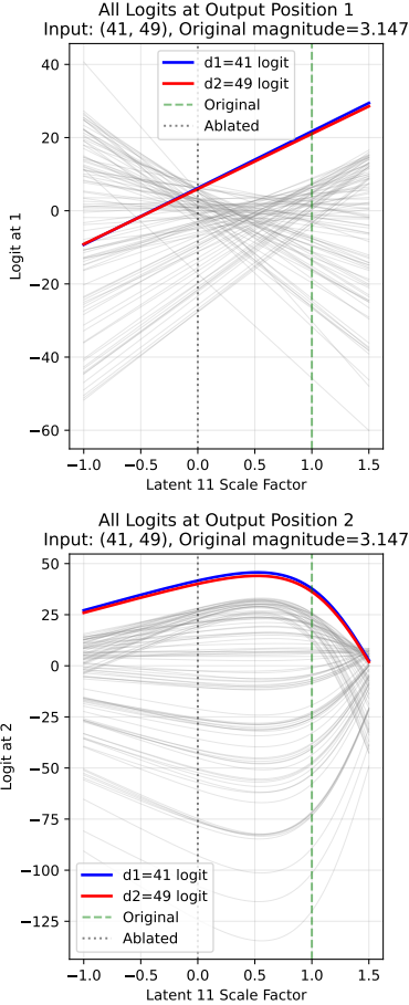
Figure 12. In the BatchTopK SAE from Section ??, latent 11 cannot be scaled to swap input bigram (41, 49) because the logit for 49 is never argmax in position o_1 , as shown by the top plot.
