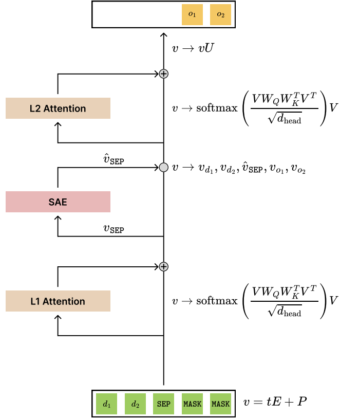
Figure 3. This diagram shows the structure of the two-layer attention-only transformer and how the SAE is used to extract and analyse the learned representations. v denotes the residual stream, which is read from and written to after each layer and has shape (5, d_{\text{model}}) . t is the vector of input tokens [d_1, d_2, \text{SEP}, \text{MASK}, \text{MASK}] , E and P are the token and position embedding matrices respectively, U is the unembedding matrix, and each attention layer has key and query matrices, K^i and Q^i respectively, for i \in [1, 2, 3] . The value and output matrices for each layer are fixed to the identity, and d_{\text{head}} = 64 . The SAE takes the residual vector at SEP, v_{\text{SEP}} , as input and patches reconstruction \hat{v}_{\text{SEP}} back into the stream. Accuracy is calculated on the final two output logits only, represented by (o_1, o_2) .
