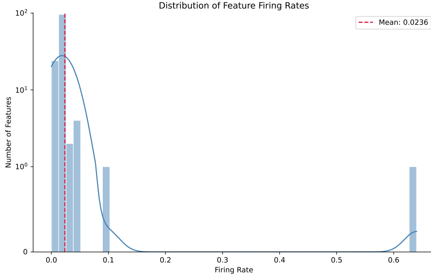
Figure 4. This histogram shows the distribution of firing rates for the SAE checkpoint’s latents. The y-axis uses a symmetric logarithmic scale with a linear scale between [-1, 1] . A given latent’s firing rate is the proportion of inputs which cause that latent to activate. The special latents are the only ones with a firing rate greater than one standard deviation from the mean (mean: 0.0236, standard deviation: 0.0559): latent 11 has rate 0.6400, latent 56 has rate 0.0991.
