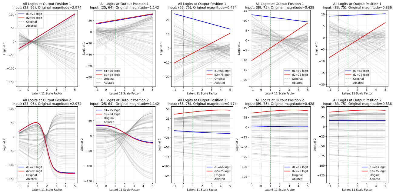
Figure 9. For 0.2% of inputs, the logit for the symbol at d_1 is always dominant at o_1 in the observed latent scale range (in the BatchTopK SAE from Section ??), so there is no scale where the the symbol at d_2 is predicted instead.
