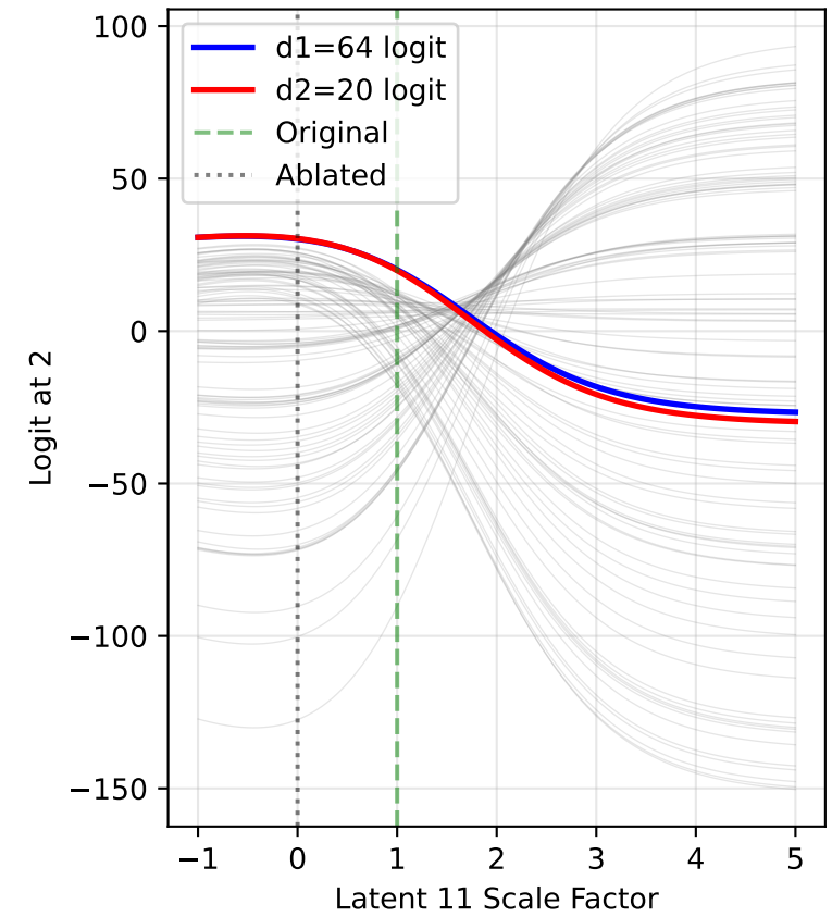
All Logits at Output Position 2 Input: (64, 20), Original magnitude=1.473
