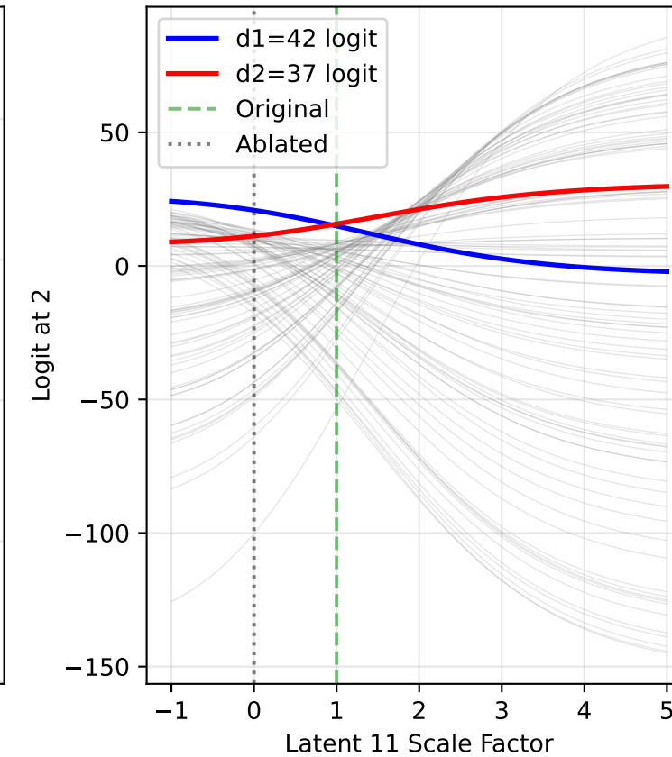
All Logits at Output Position 2 Input: (42, 37), Original magnitude=0.911
