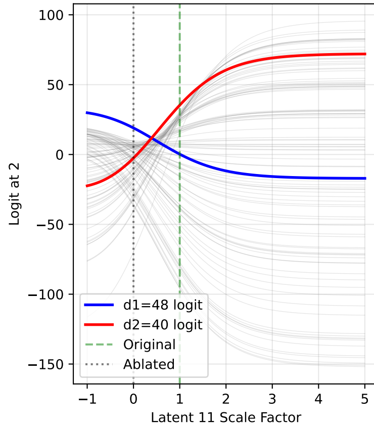
All Logits at Output Position 2 Input: (48, 40), Original magnitude=1.510
