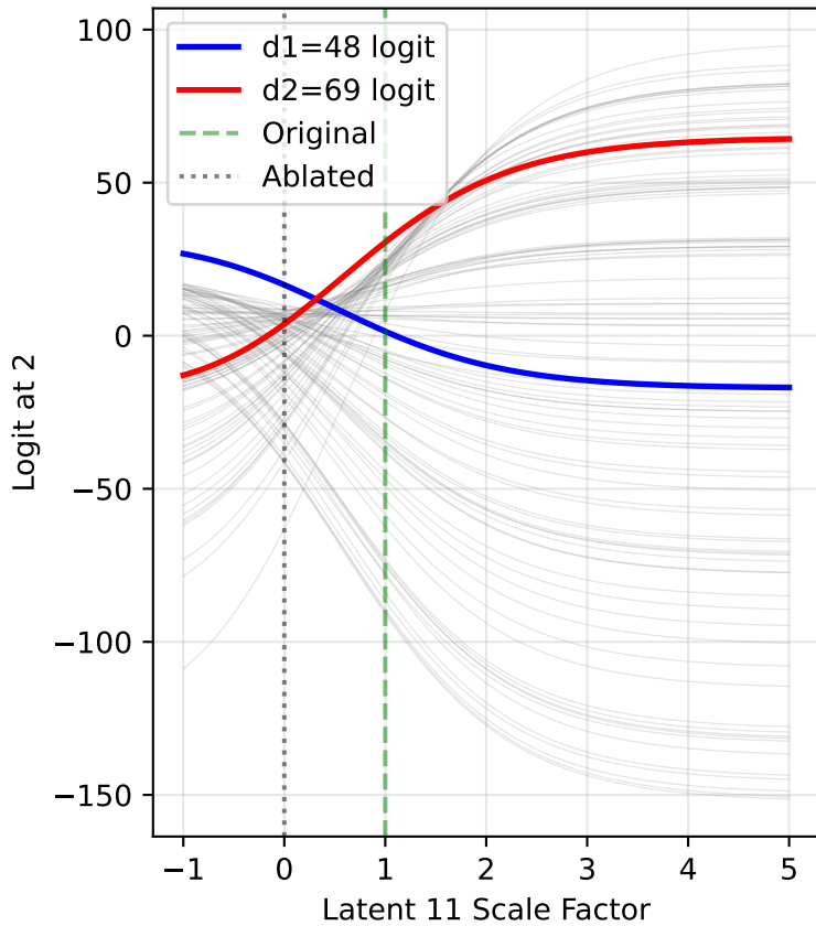
All Logits at Output Position 2 Input: (48, 69), Original magnitude=1.243
