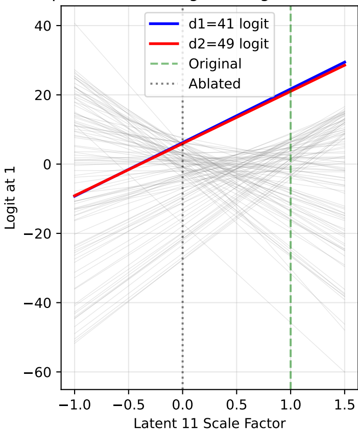
All Logits at Output Position 1 Input: (41, 49), Original magnitude=3.147
