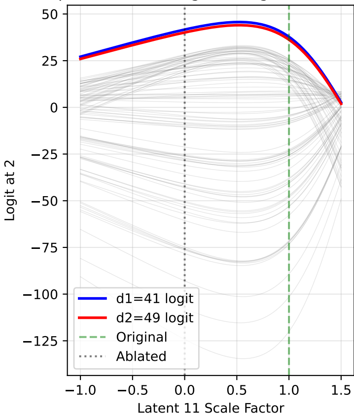
All Logits at Output Position 2 Input: (41, 49), Original magnitude=3.147
