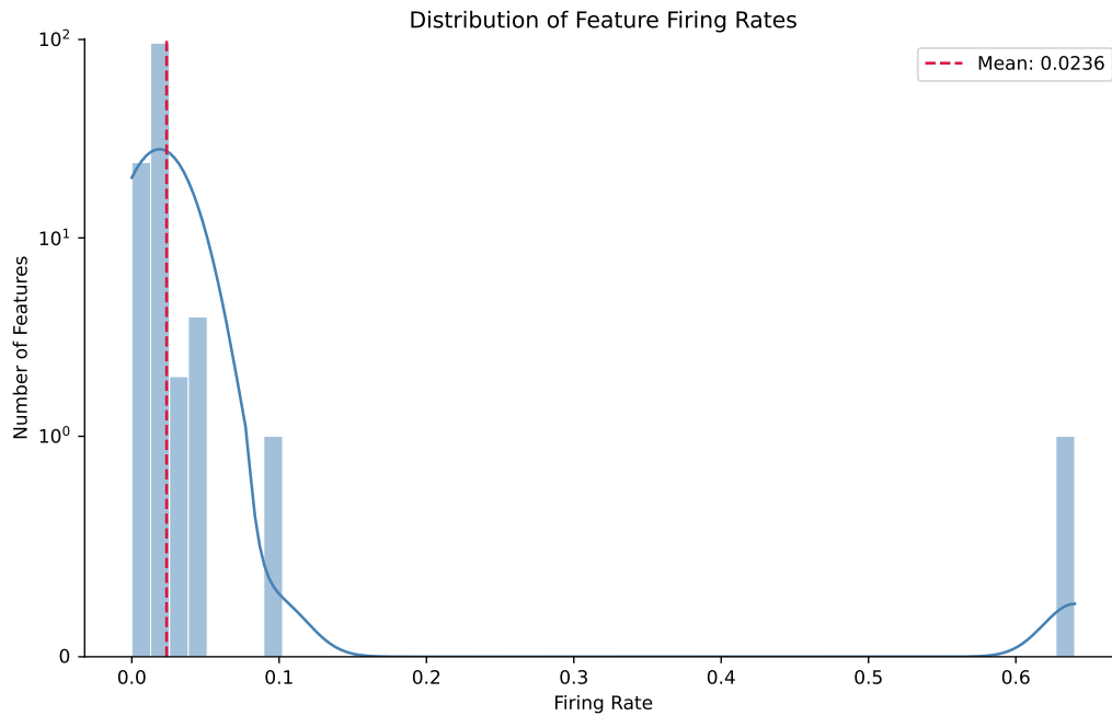
Figure 5. This histogram shows the distribution of firing rates for the SAE checkpoint’s latents. The y-axis uses a symmetric logarithmic scale with a linear scale between [-1, 1] . A given latent’s firing rate is the proportion of inputs which cause that latent to activate. The special latents are the only ones with a firing rate greater than one standard deviation from the mean (mean: 0.0236, standard deviation: 0.0559): latent 11 has rate 0.6400, latent 56 has rate 0.0991.
